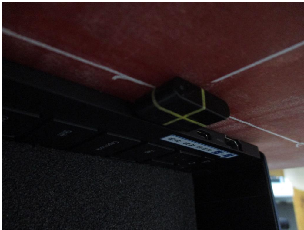
Horizontal-Down from Flat Phantom (Separation Distance: 0 cm) – without USB Cable
