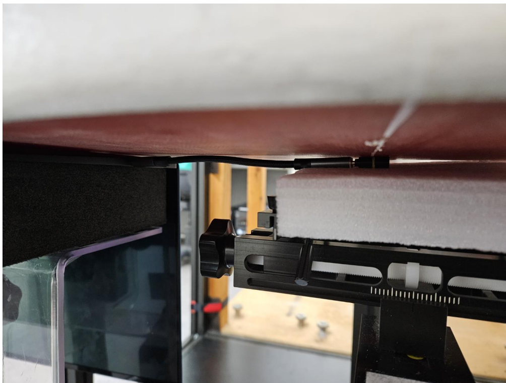
Horizontal-Down from Flat Phantom (Separation Distance: 0 cm)
