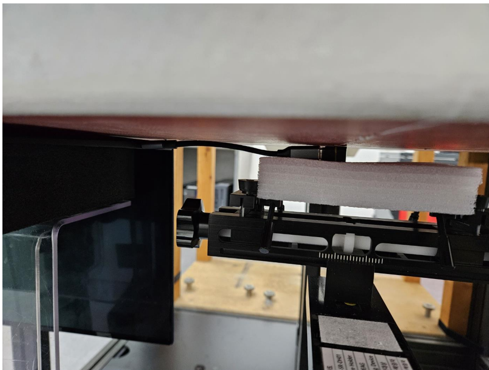
Vertical-Front from Flat Phantom (Separation Distance: 0 cm)
