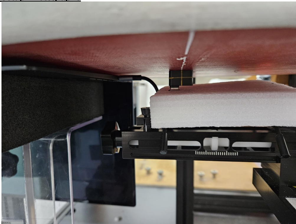
Tip of dongle from Flat Phantom (Separation Distance: 0 cm)
