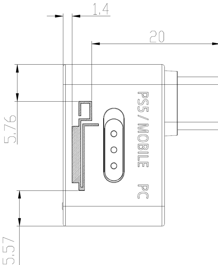
Figure E-1 Antenna Location (Front Side View)
