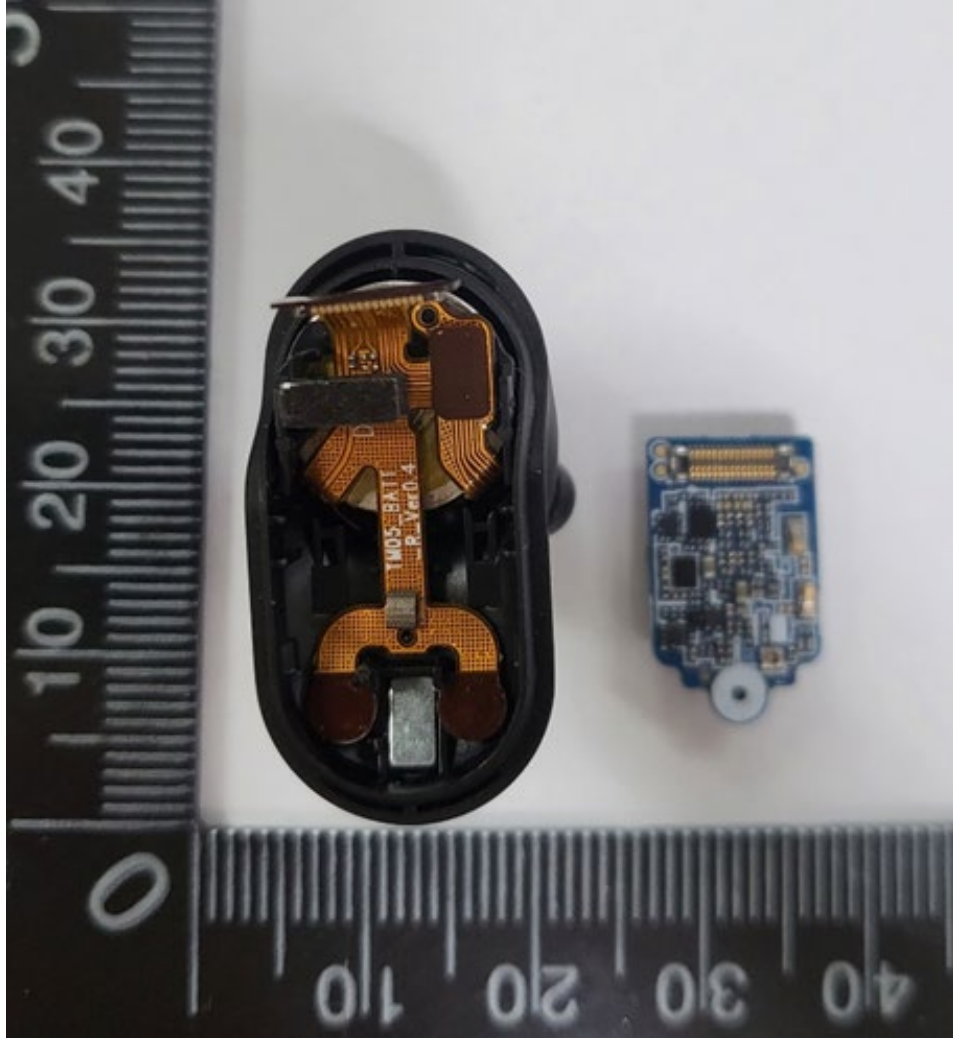
Earbuds R-CH Board
