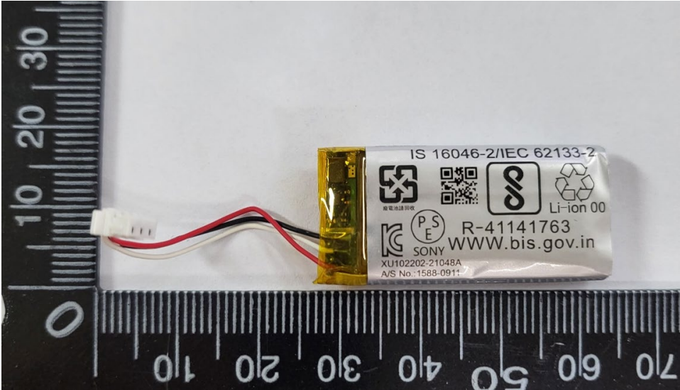
Case Battery (VDL)
