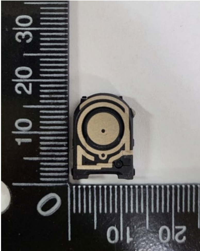
Earbuds R-CH _ LDS Antenna
