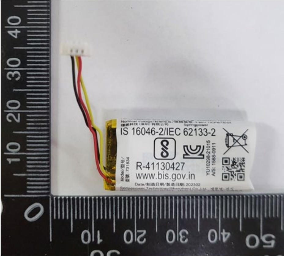
Case Battery (High Power)
