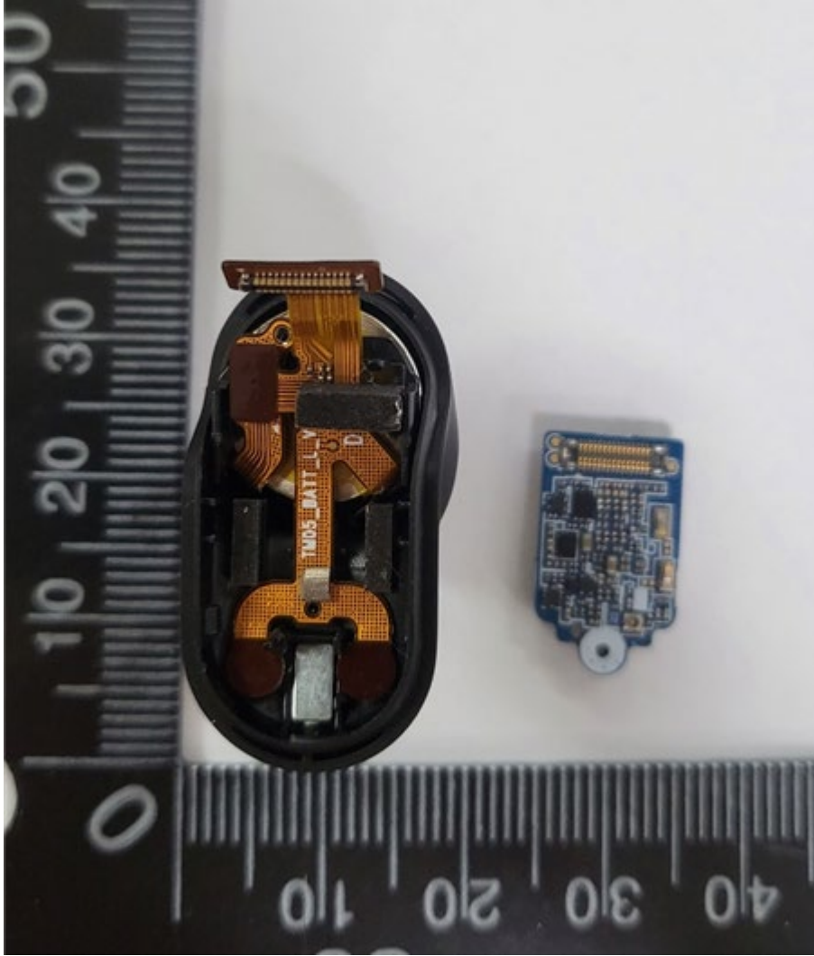
Earbuds L-CH Board
