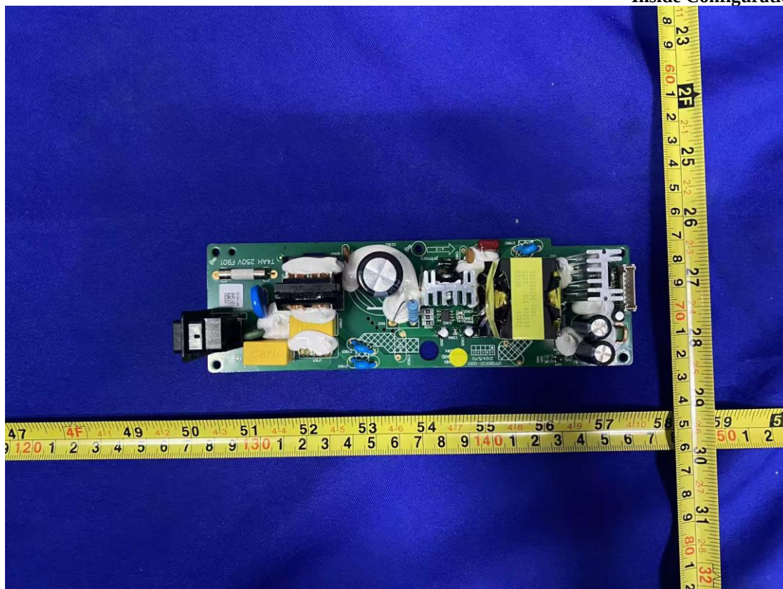
Figure 6 Inside Configuration of the EUT
