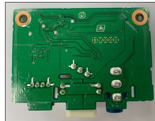
GPS PWB ( Back Side )
