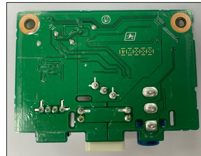
GPS PWB ( Back Side )
