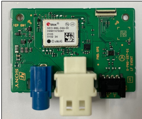
GPS PWB ( Front Side )
