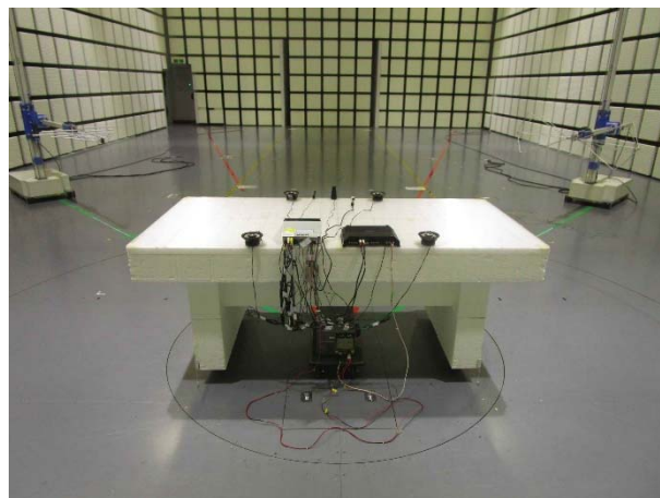
Rear(Below 1 GHz)
