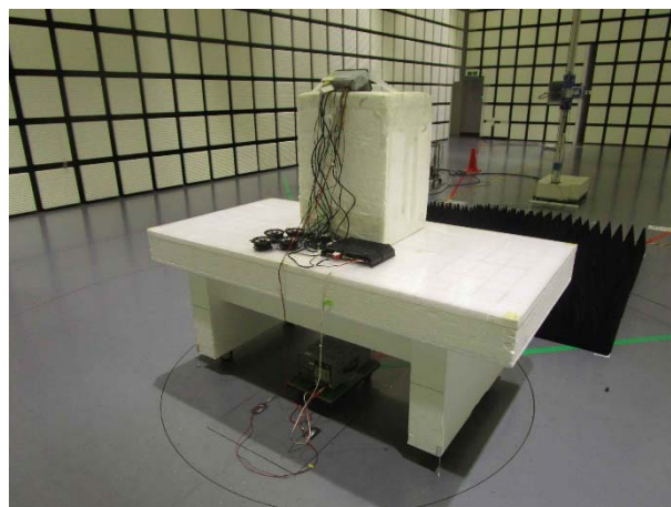
Rear(Above 1 GHz)
