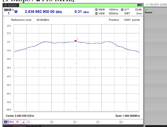
[1 Mbps / 2440 MHz]
