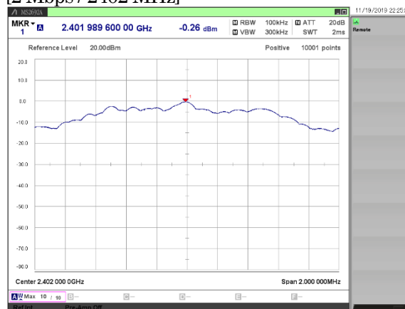
[2 Mbps / 2402 MHz]
