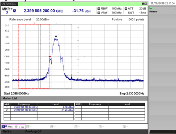
[2 Mbps / 2402 MHz]
