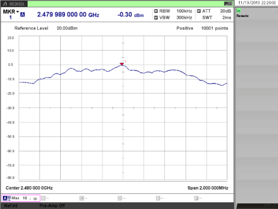
[2 Mbps / 2480 MHz]
