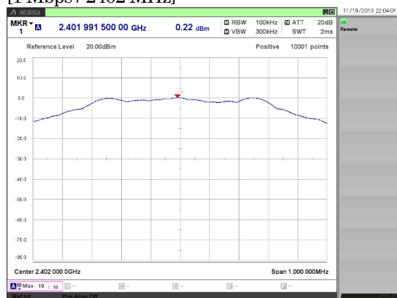
[1 Mbps / 2402 MHz]
