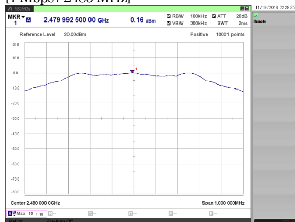
[1 Mbps / 2480 MHz]
