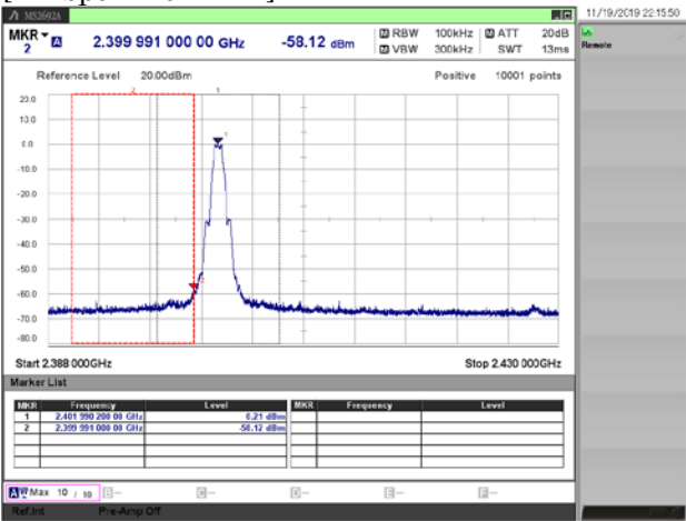
[1 Mbps / 2402 MHz]
