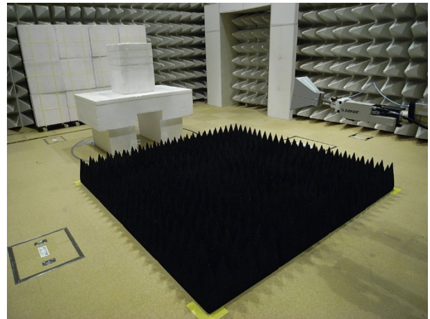
Above 1 GHz
