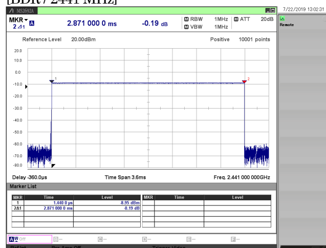
[BDR / 2441 MHz]
