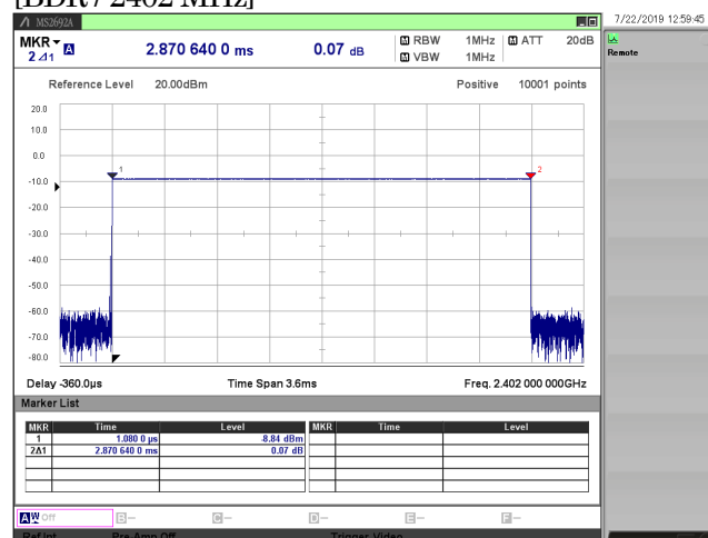
[BDR / 2402 MHz]
