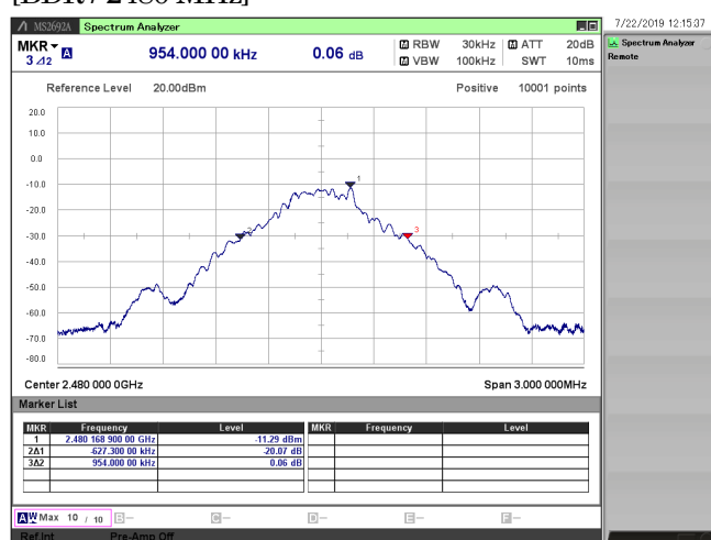
[BDR / 2480 MHz]
