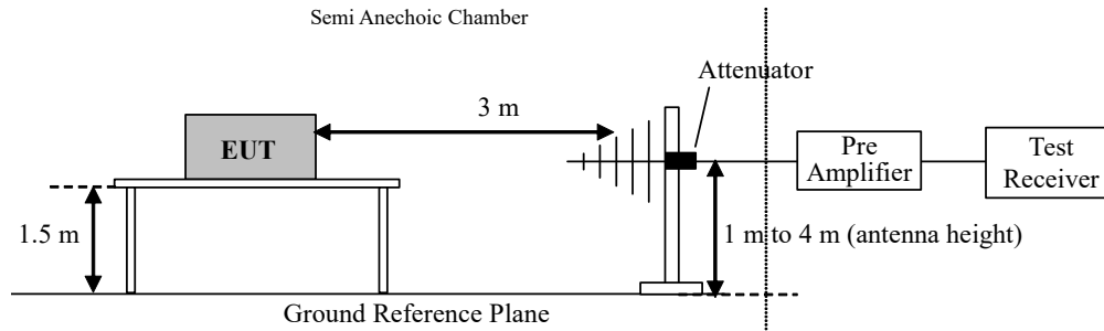
Figure 1: Test Setup
