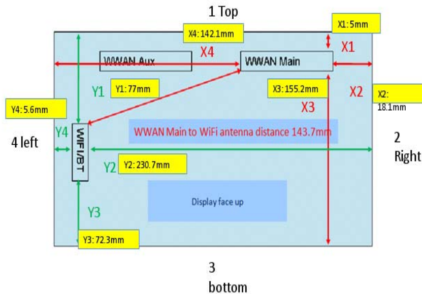
Fig.9 Antenna position of EUT
