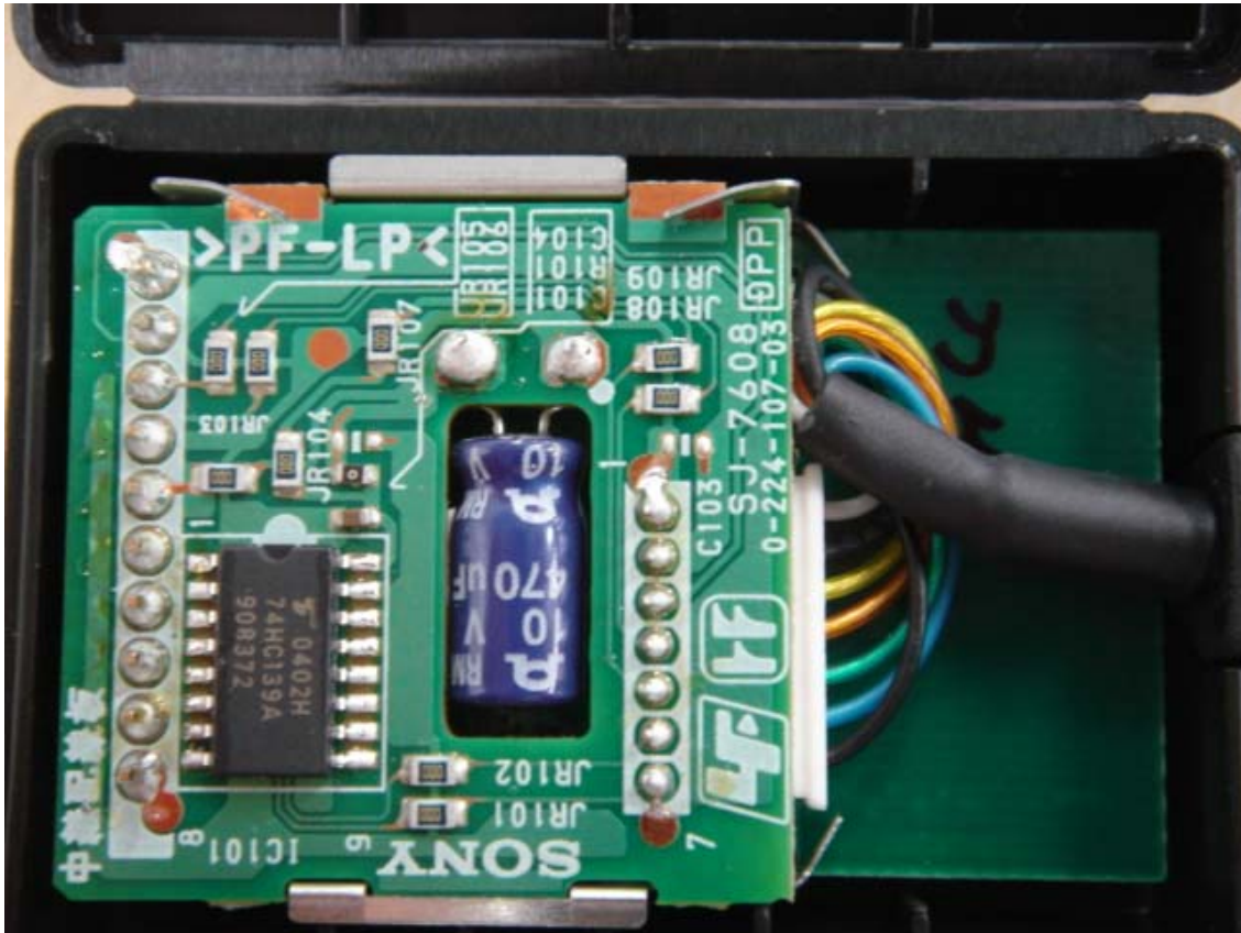
Transmitter Module cover opened
