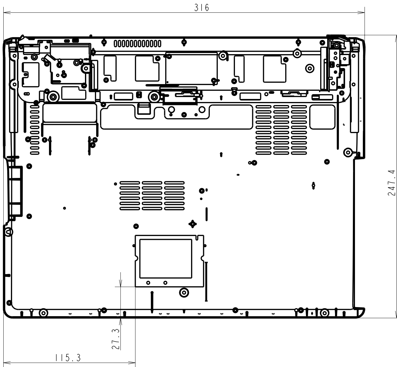
Bottom View
