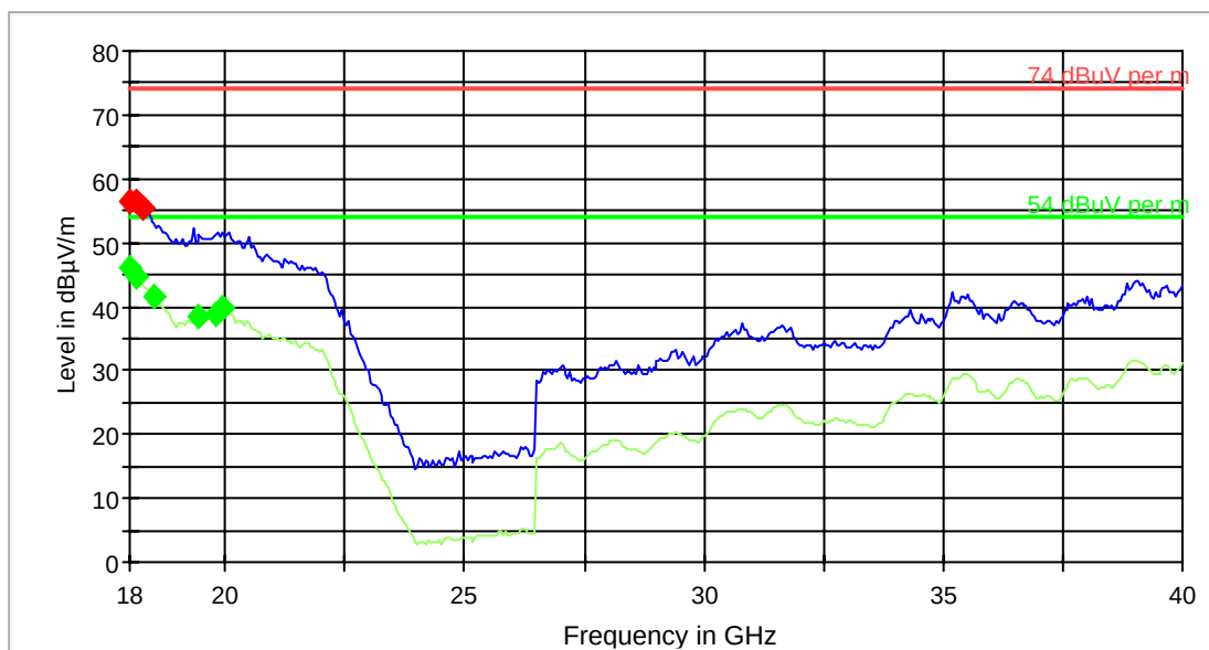
FCC 15 18-40GHz
