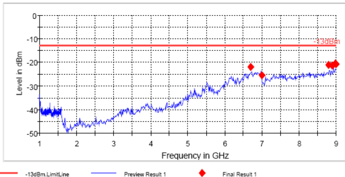
FCC 22 1-9GHz
