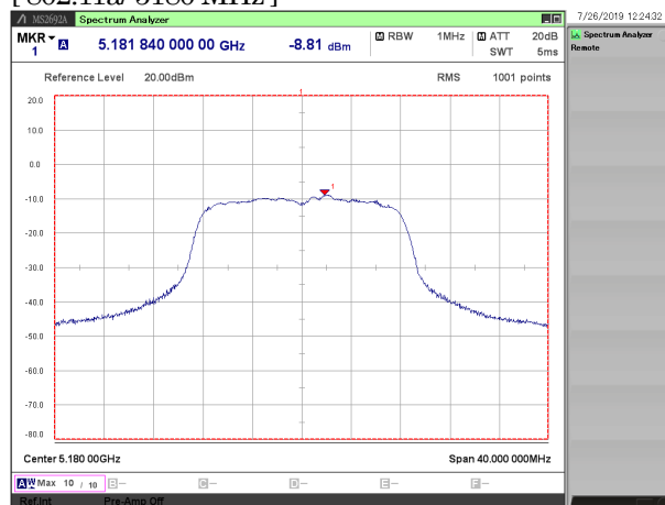
[ 802.11a/ 5180 MHz ]
