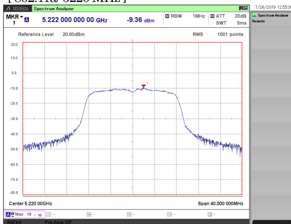
[ 802.11a/ 5220 MHz ]
