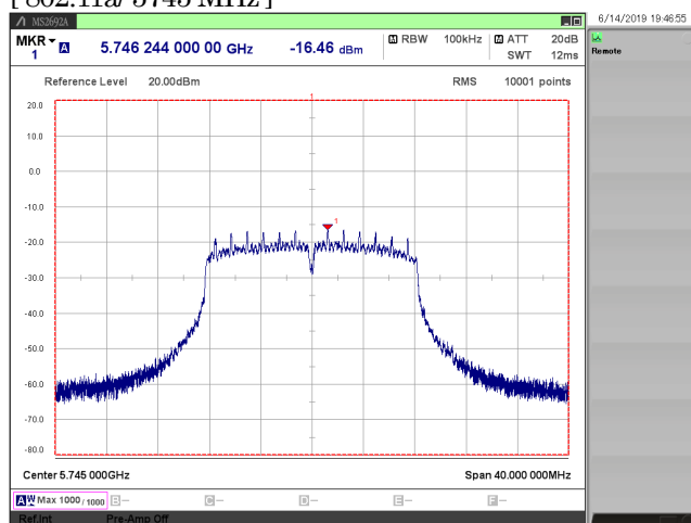
[ 802.11a/ 5745 MHz ]
