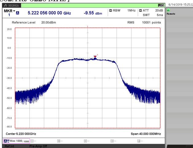
[ 802.11a/ 5220 MHz ]
