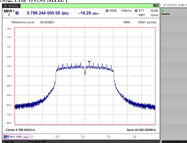
[ 802.11a/ 5785 MHz ]
