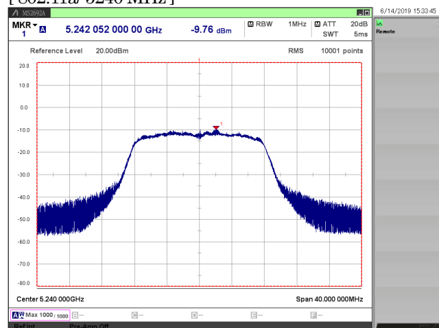
[ 802.11a/ 5240 MHz ]
