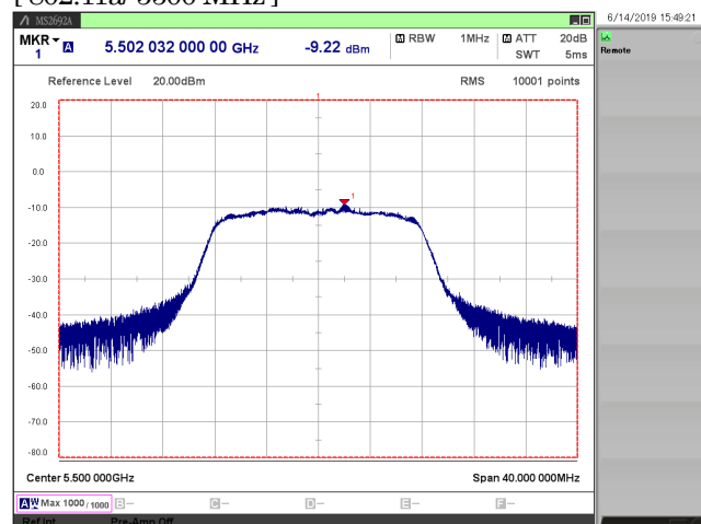
[ 802.11a/ 5500 MHz ]
