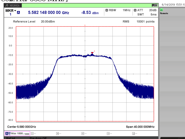
[ 802.11a/ 5580 MHz ]
