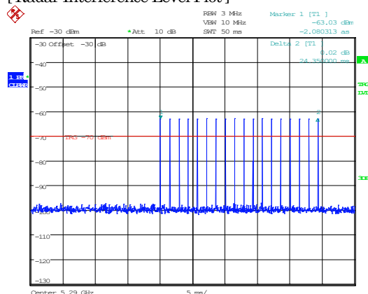
[ Radar Interference Level Plot ]
