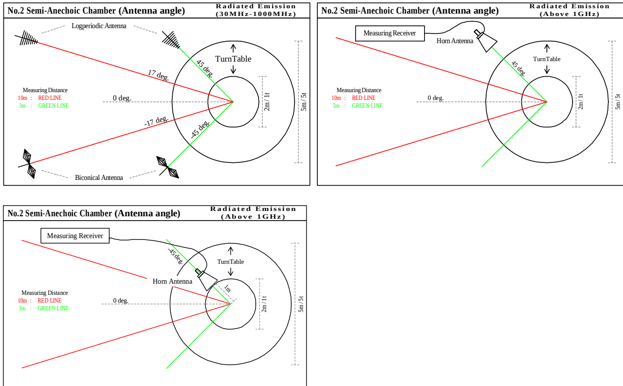
Figure 1. Antenna angle
