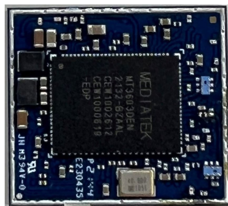
Top (w/o shielding cover)
