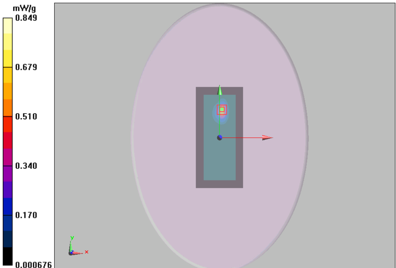
Figure 10 802.11b Test Position 2 Channel 1
