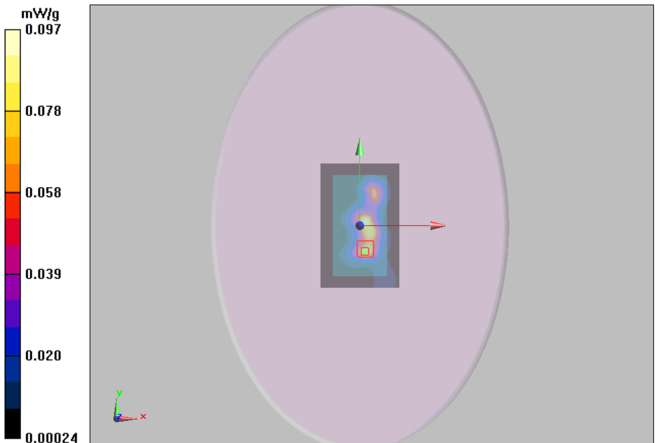
Figure 11 802.11b Test Position 5 Channel 6
