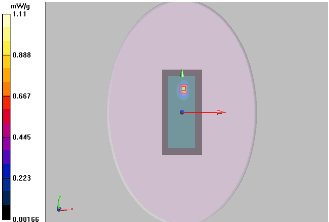
Figure 9 802.11b Test Position 2 Channel 6
