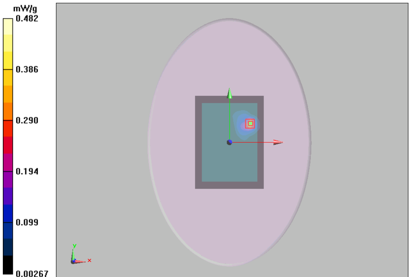
Figure 7 802.11b Test Position 1 Channel 6
