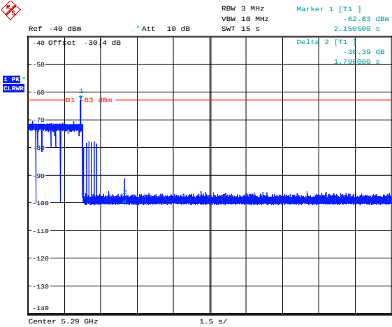
[ Channel Move Time / Channel Closing Transmission Time Plot ]
