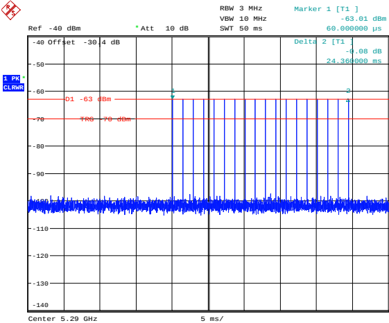
[ Radar Interference Level Plot ]
