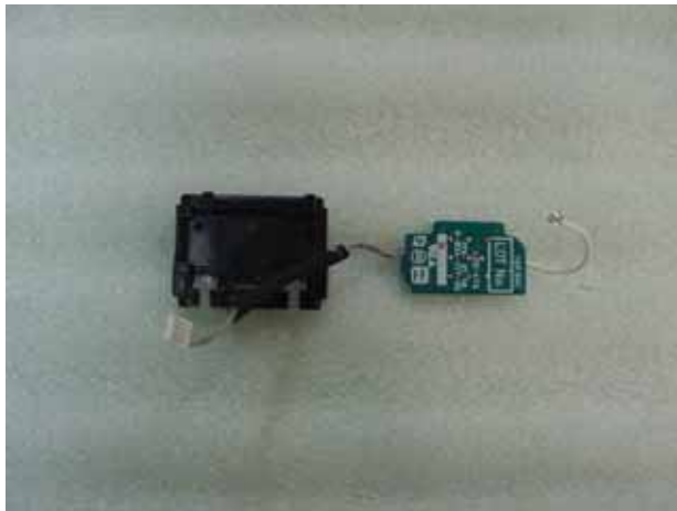
Fig.21 Detach LED-470
