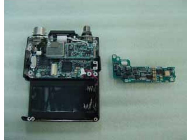
Fig.02 Detach AU-319
