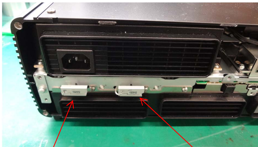
WLAN ANTENNA
