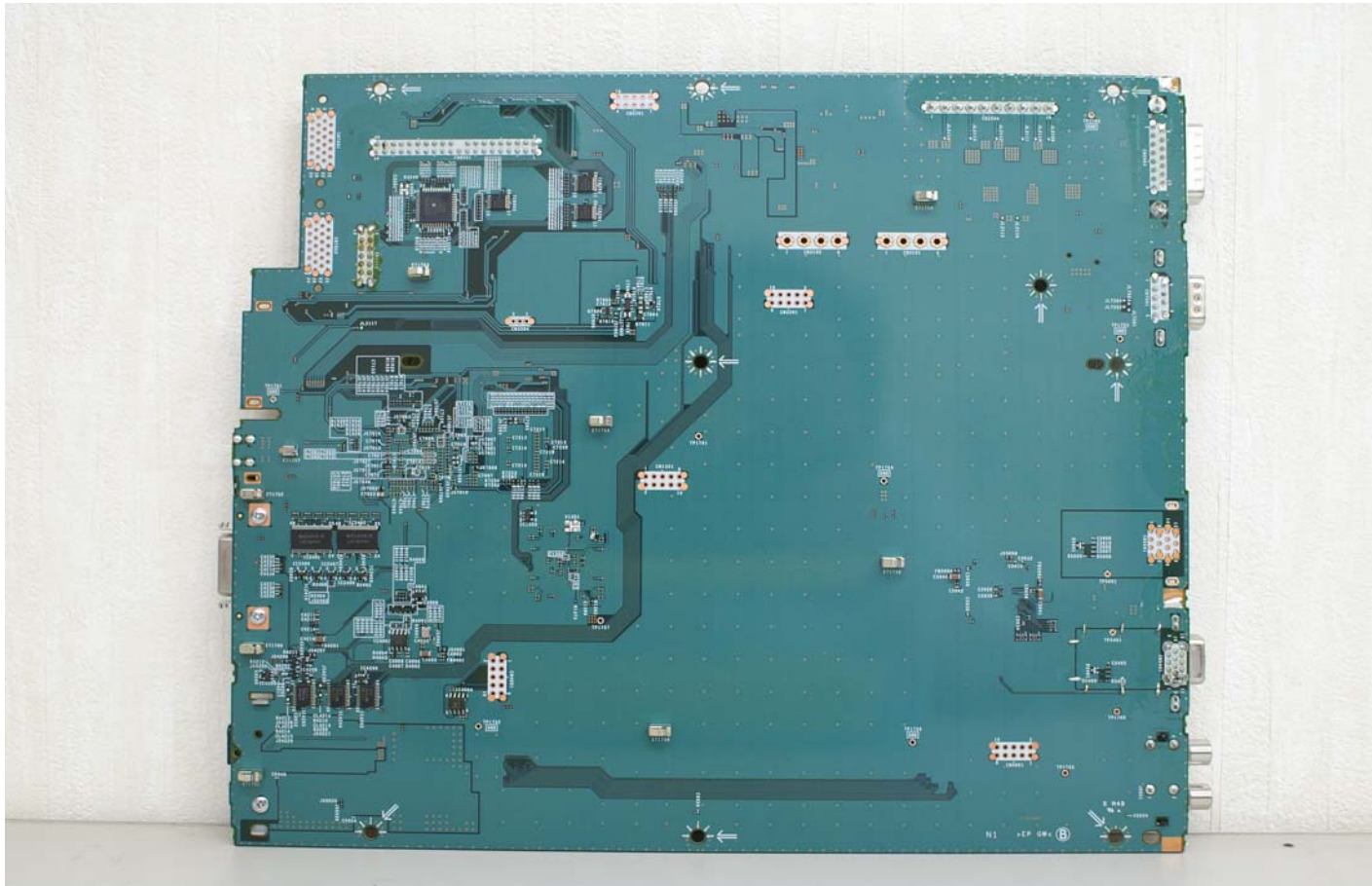
TMU-002 PWB (2/2)
