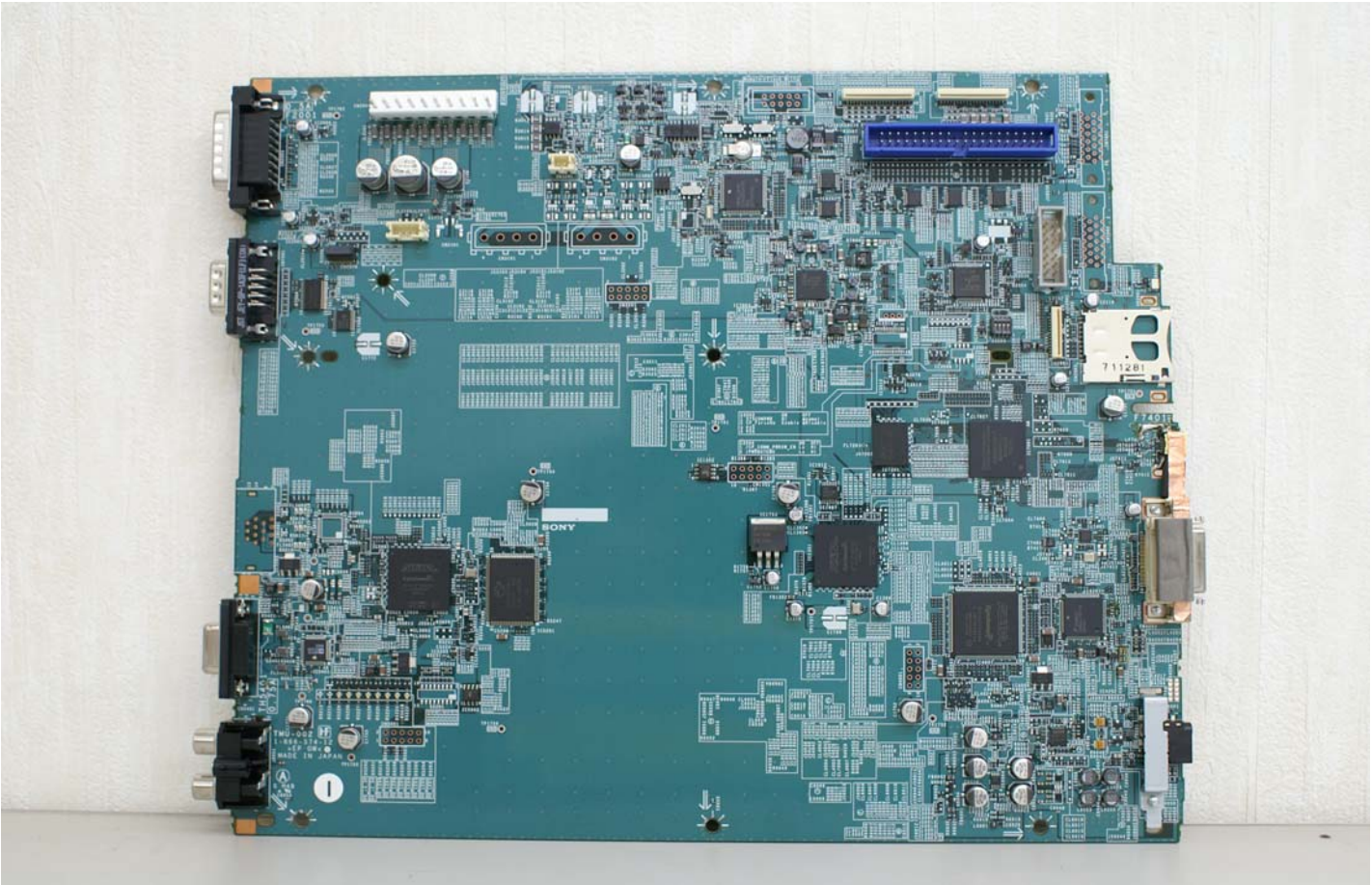
TMU-002 PWB (2/2)
