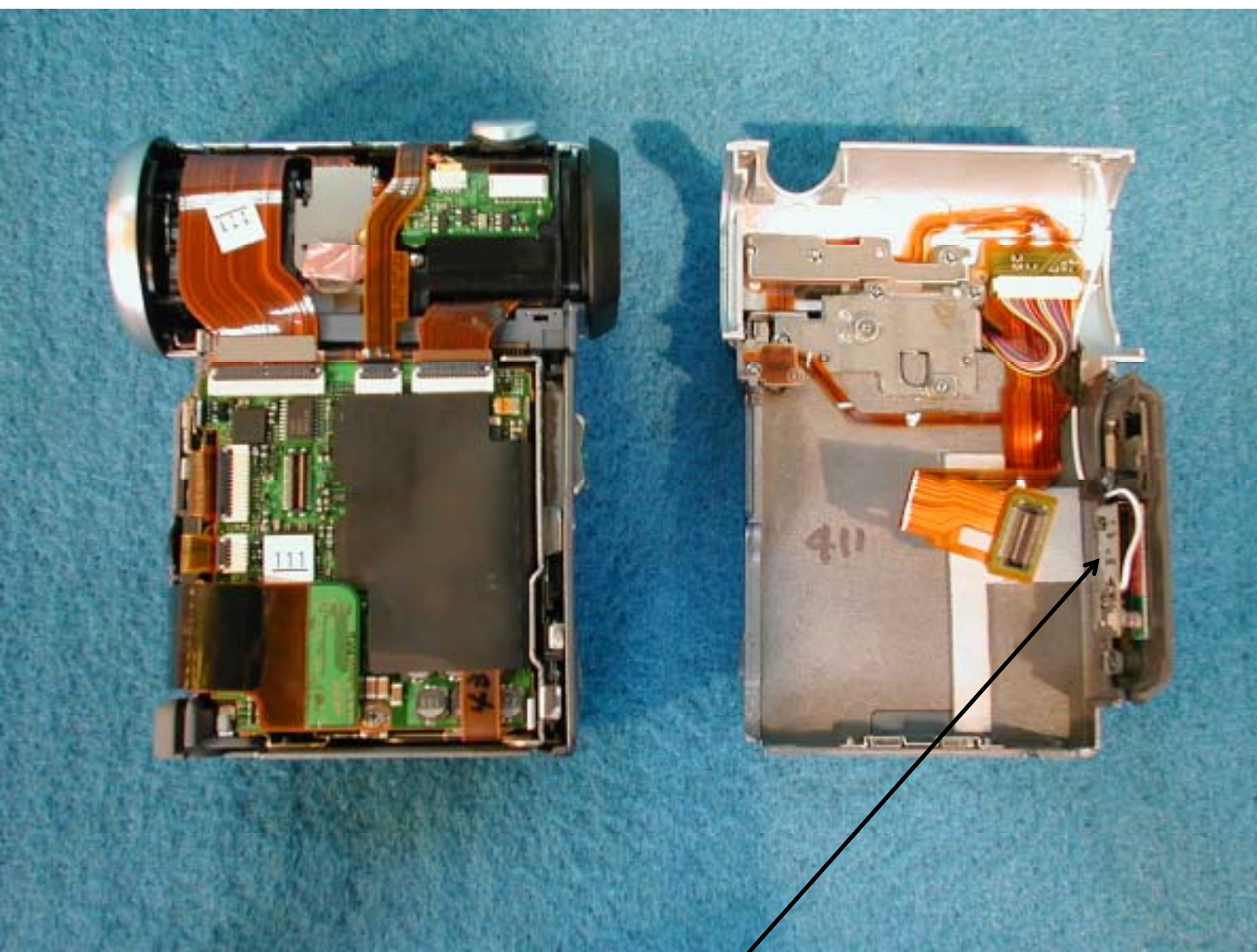
Antenna Position
