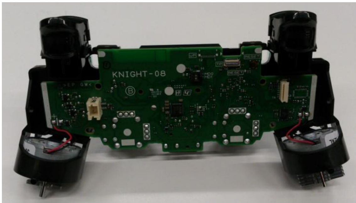
Photo 10Inside(4/5)/ Location of Antenna &Module
