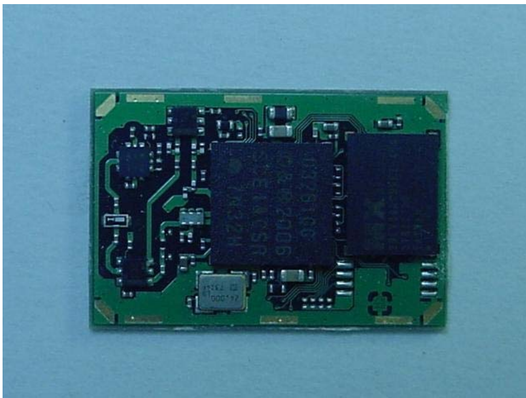
Top of BT Module without Shield Case
