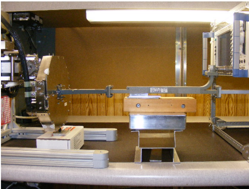
Figure G-6 – Spurious Emissions at Antenna Terminal Test Setup (12.4 – 18 GHz)
