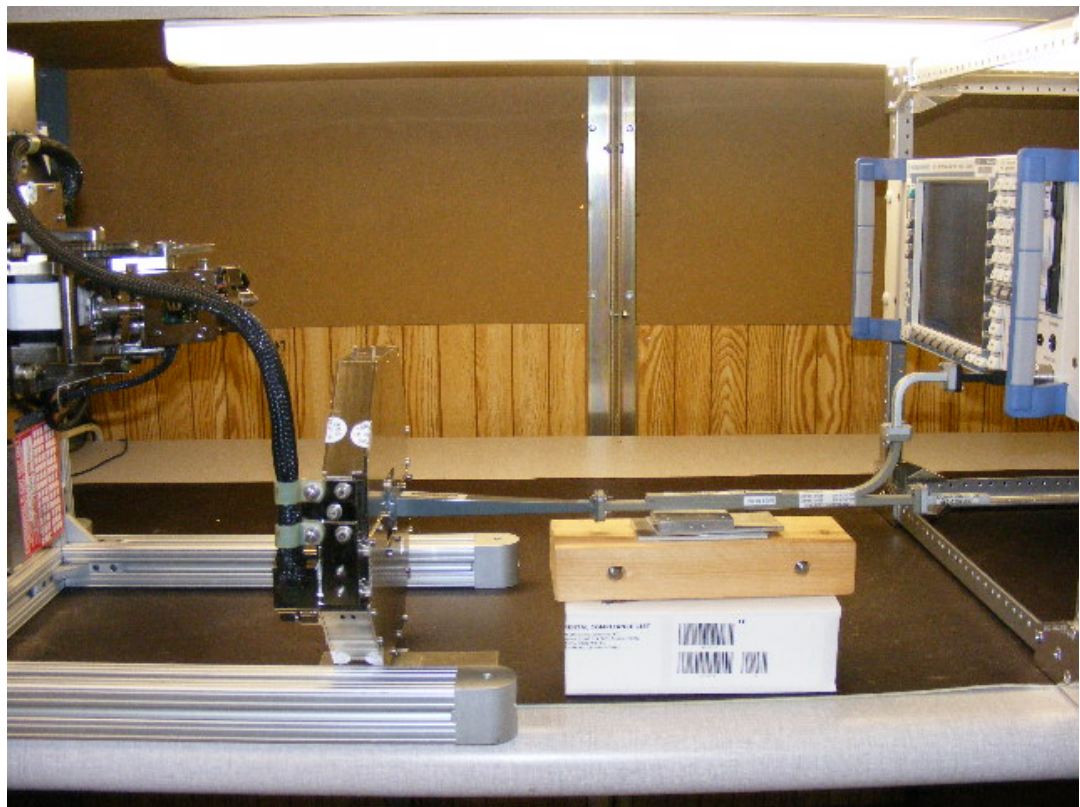
Figure G-8 – Spurious Emissions at Antenna Terminal Test Setup (26.5 – 40 GHz)
