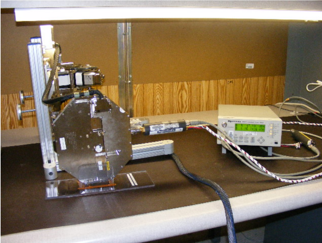
Figure G-1 – RF Power Output Test Equipment Setup
