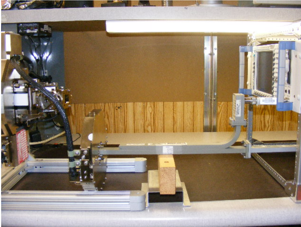
Figure G-5 – Spurious Emissions at Antenna Terminal Test Setup (8.2 – 12.4 GHz)
