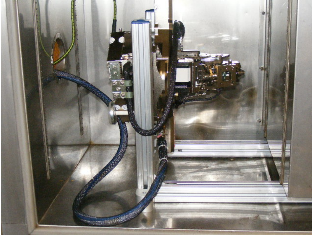
Figure G-3 – Frequency Stability Test Setup 2
