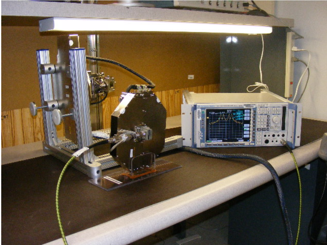
Figure G-4 – Occupied Bandwidth Test Setup
