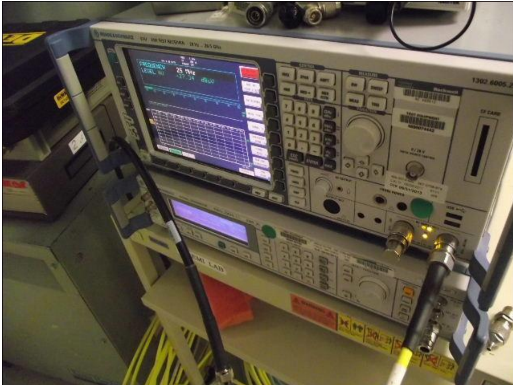
Figure G-5 – Radiated Spurious Emissions Test Setup 3
