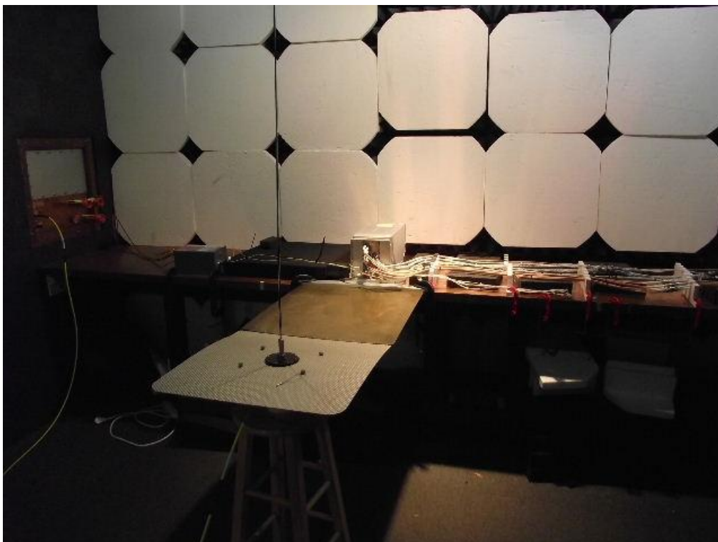
Figure G-9 – Radiated Spurious Emissions Test Setup, 150 kHz – 20 MHz, Vertical Polarization
