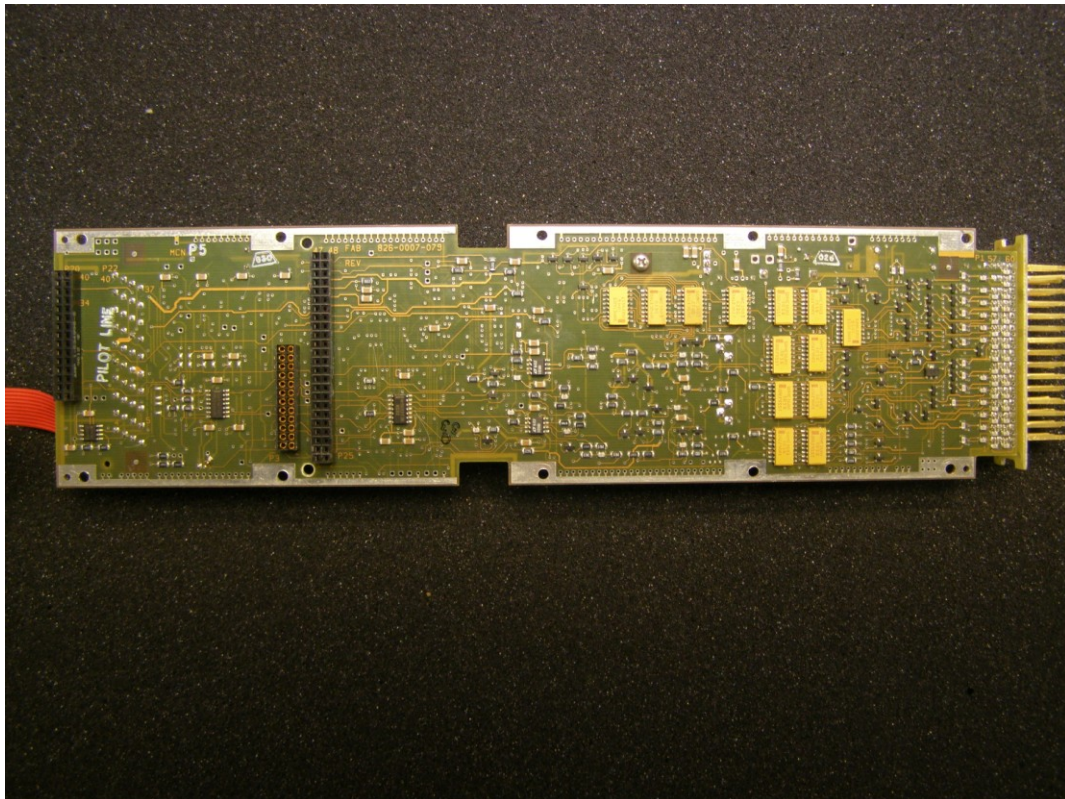
VIDEO MODULE – BOTTOM VIEW
