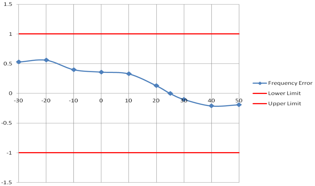
Frequency Stability vs Temperature
