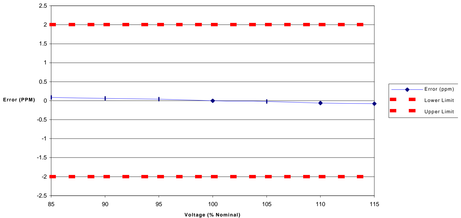
Frequency Error vs Supply Voltage
