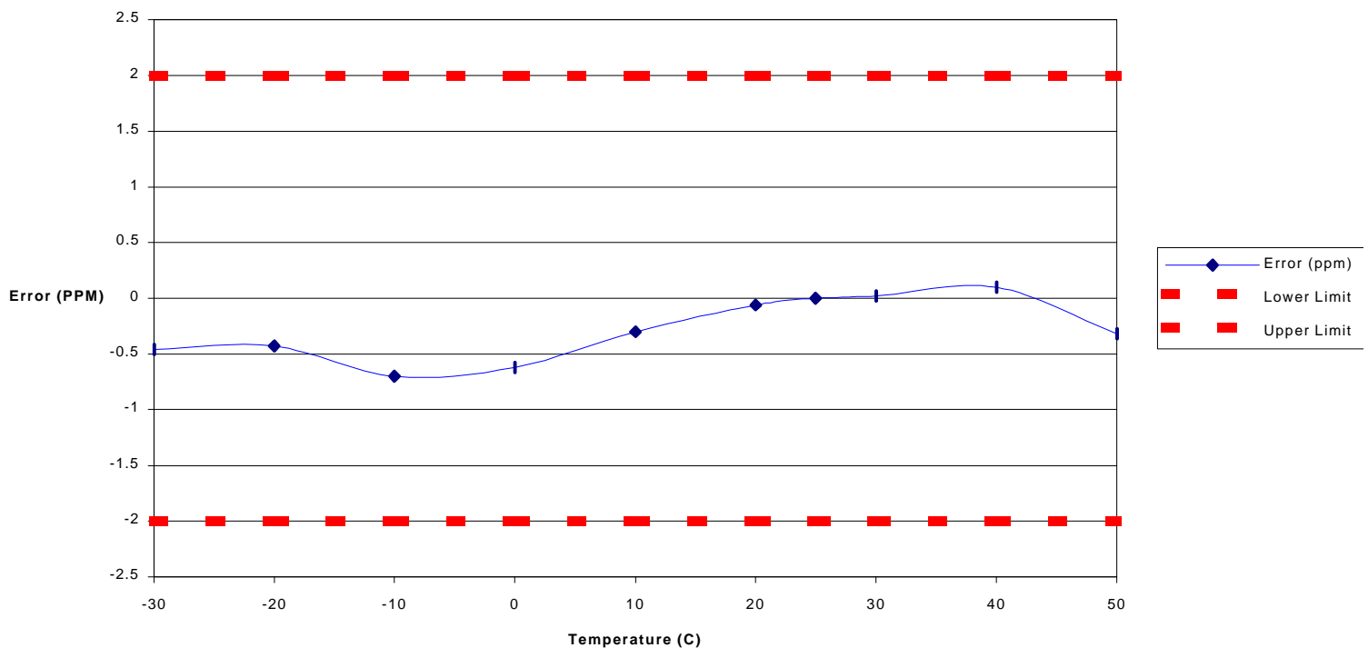
Frequency Error vs Temperature
