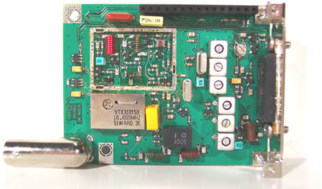
RF Board-Top View
