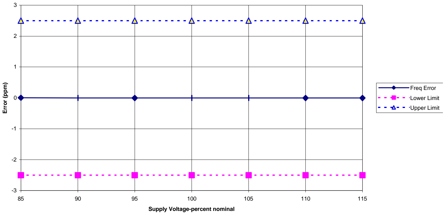
Frequency Error vs Supply Voltage
