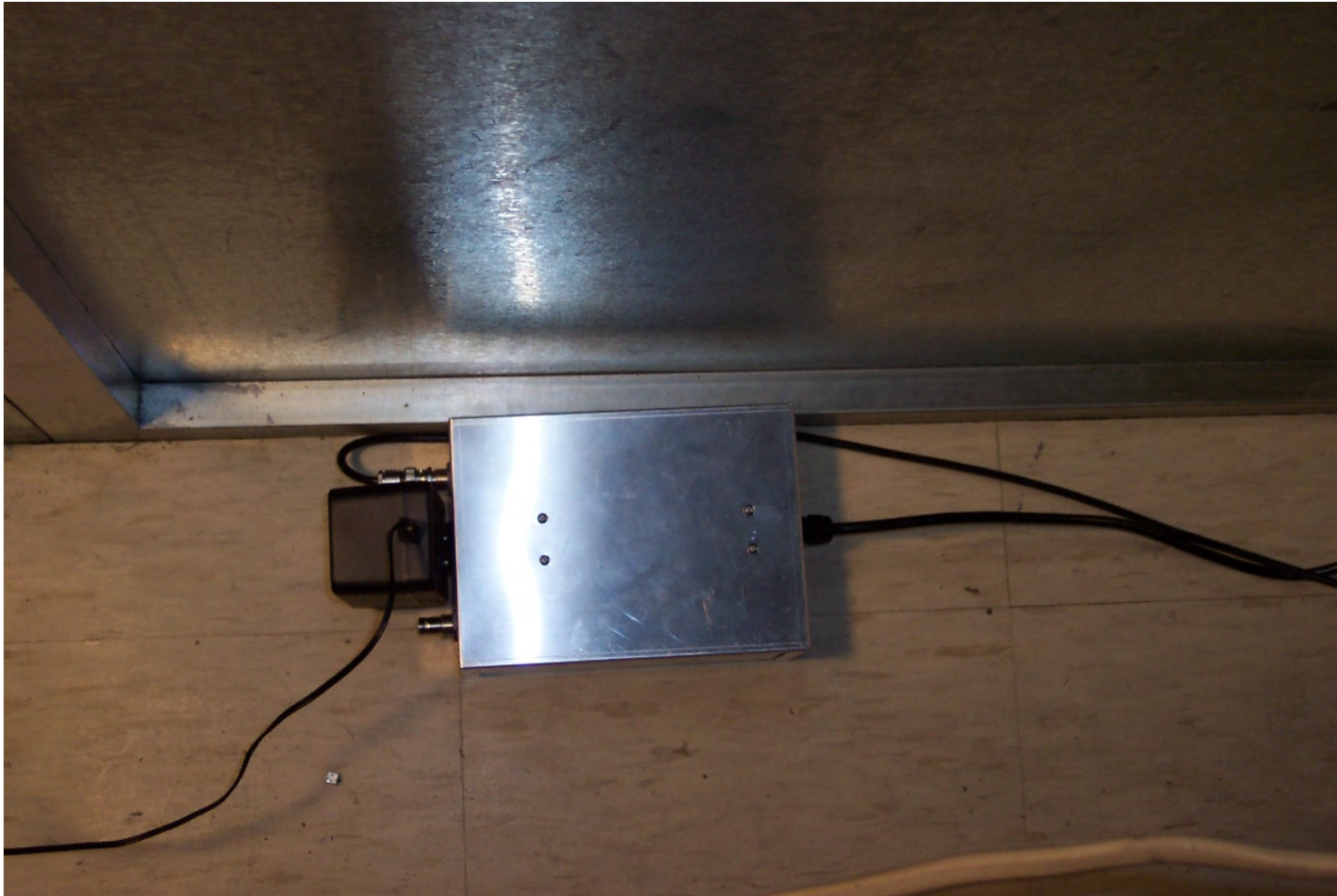
Line impedance stabilization network on floor of AC powerline conducted test site
