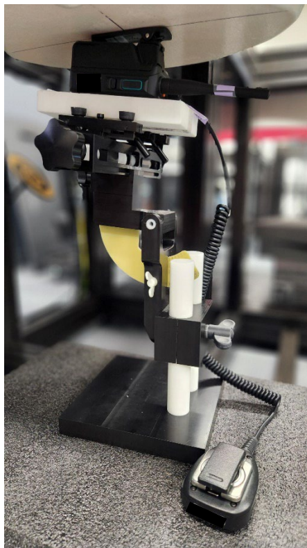
Figure E SAR Test Setup – Body– Back 0mm Battery BP-291 with Belt Clip, Audio Accessory HM-222HLS
