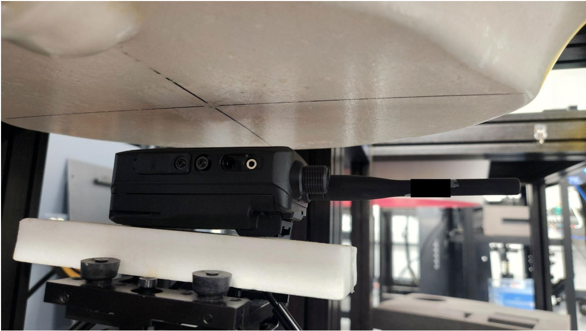
Figure C SAR Test Setup – Face – Front 25mm, Battery BP-315
