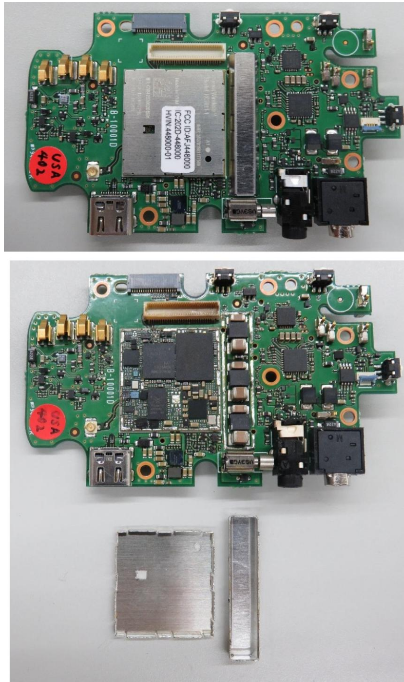
MAIN Board side-A view
