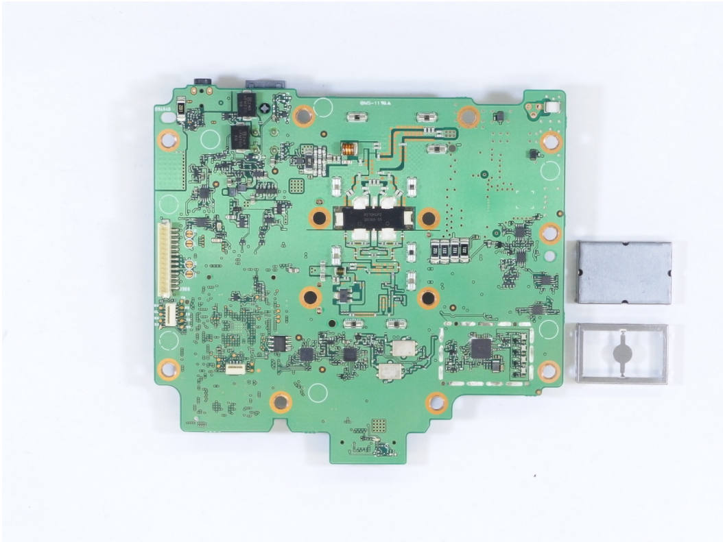
IC-F6330D MAIN unit Main board side-A
