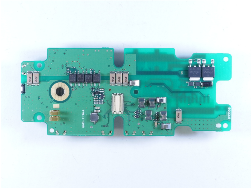
IC-F6330D MIC unit PD board side-A
