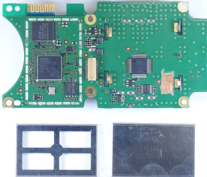
IC-F6330D MIC unit Logic board side-B
