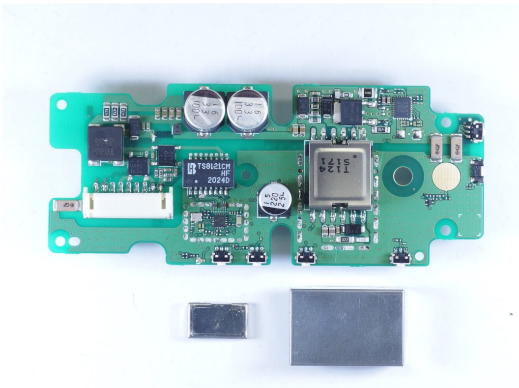
IC-F6330D MIC unit PD board side-B
