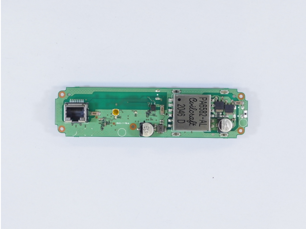
IC-F6330D MAIN unit Front board side-A
