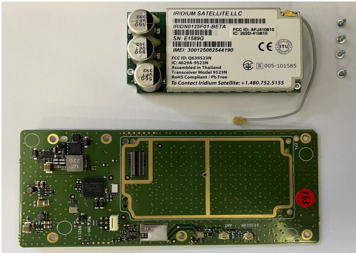
ANTENNA UNIT RF BOARD (SIDE A)
