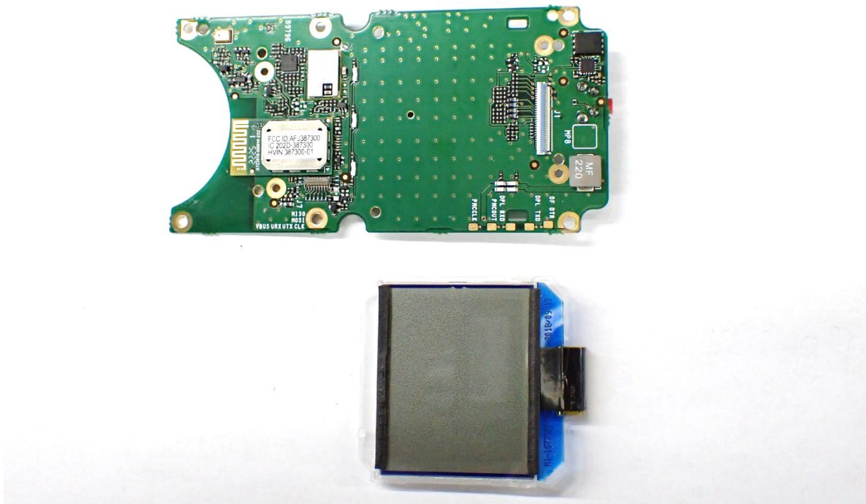
FRONT UNIT BOARD (SIDE A)
