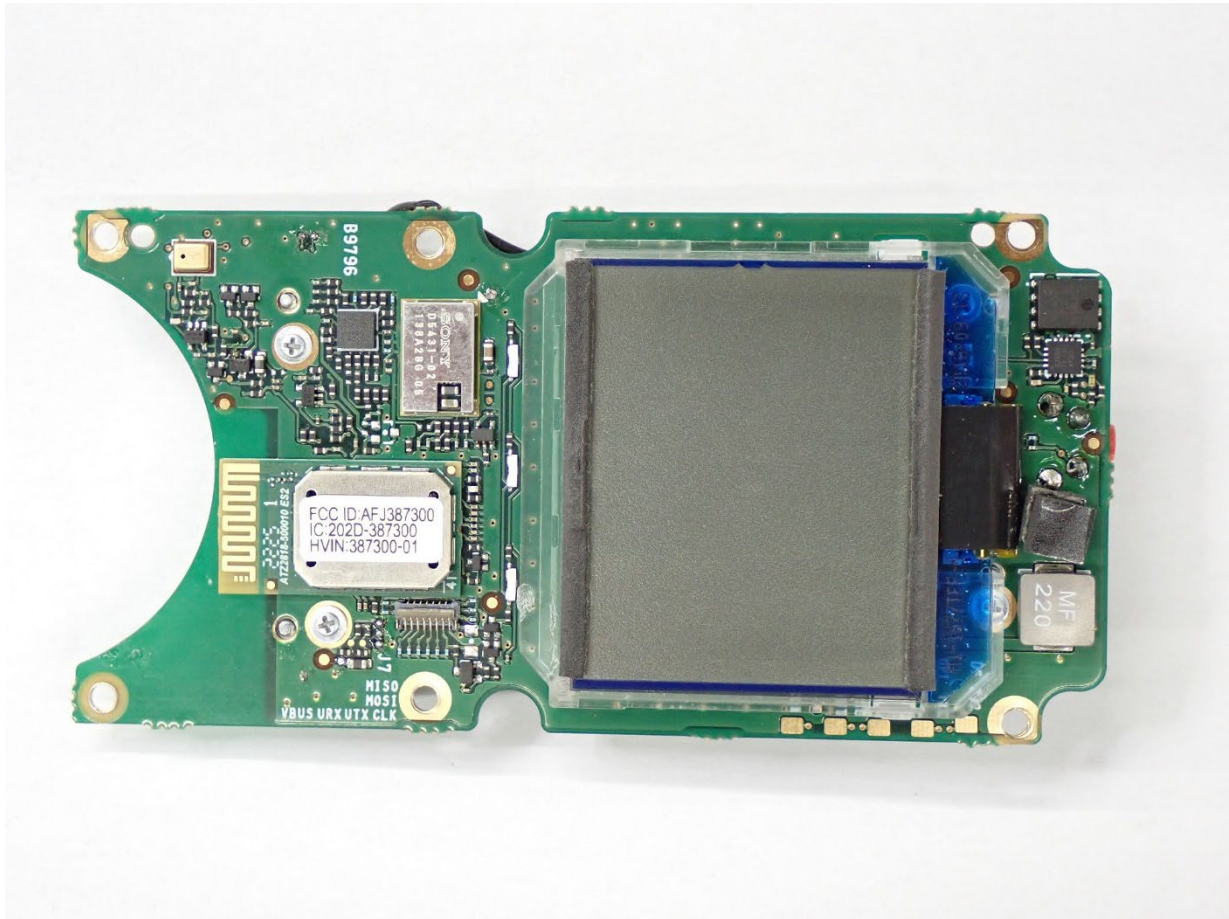
FRONT UNIT with LCD attached (SIDE A)
