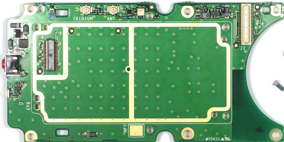
FRONT UNIT BOARD (SIDE B)
