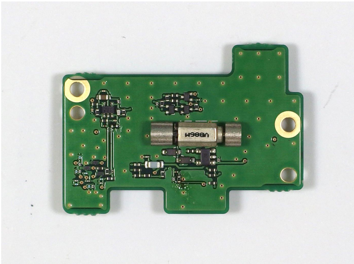
CONTACT UNIT BOARD (SIDE B)
