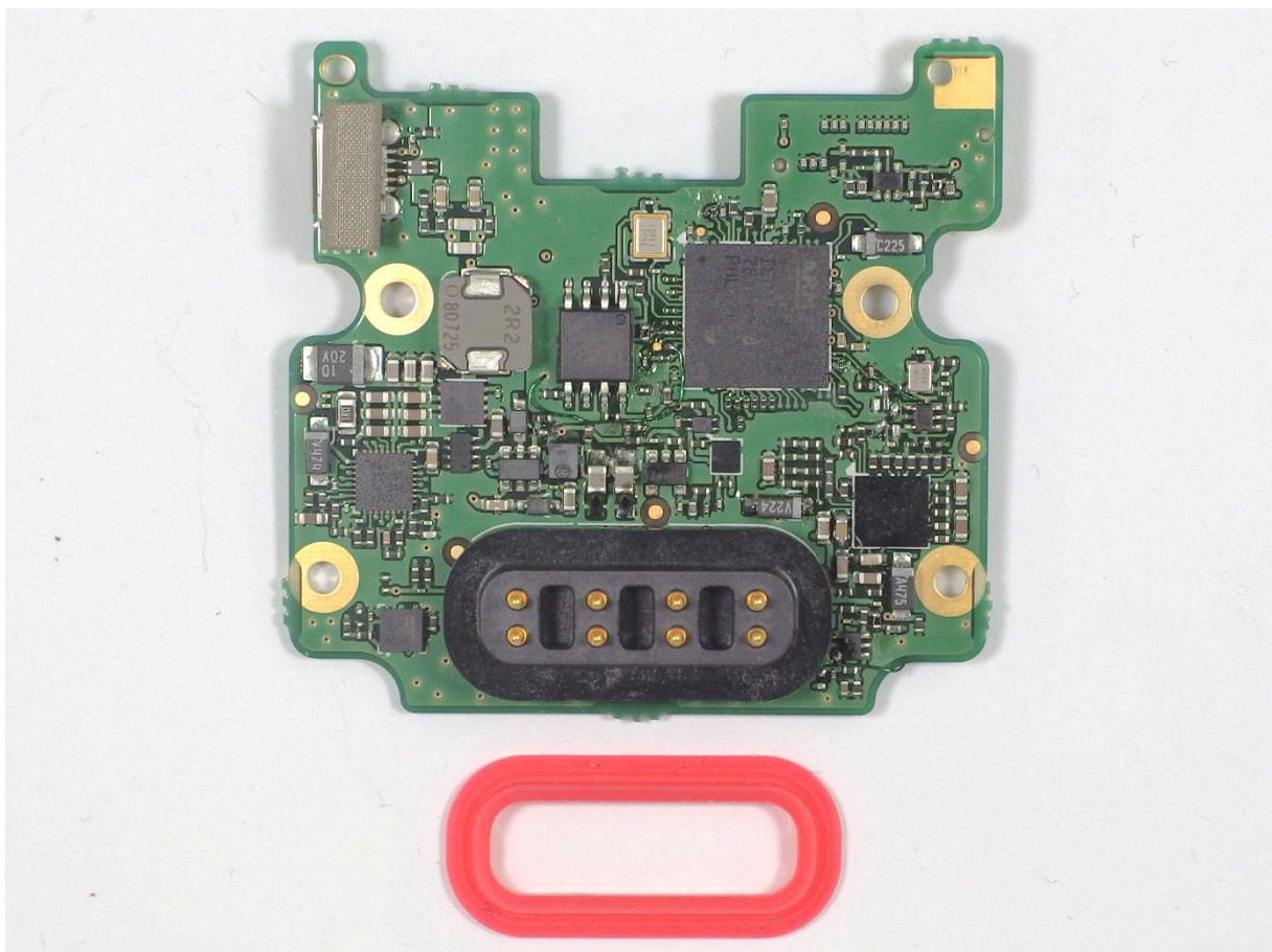
MAIN UNIT (SIDE B)
