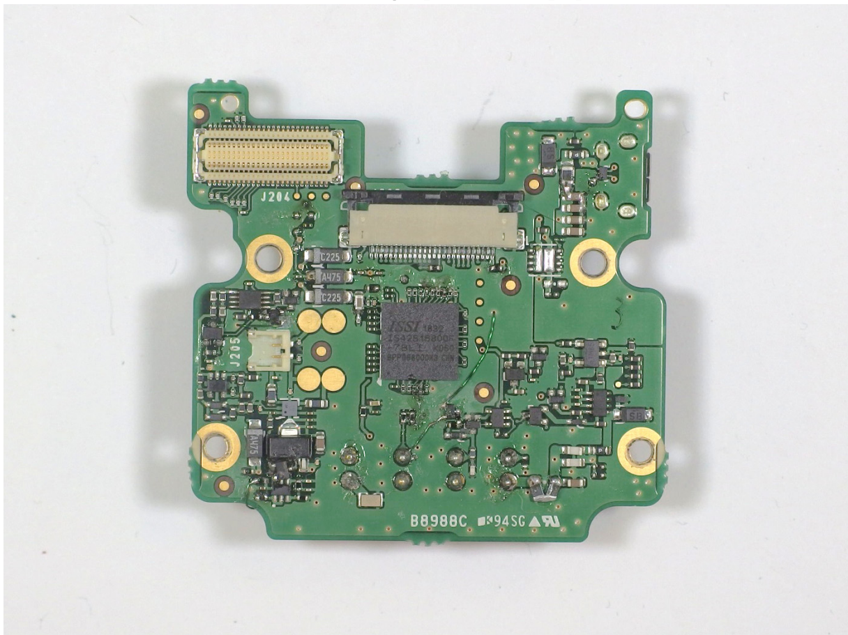
MAIN UNIT (SIDE A)
