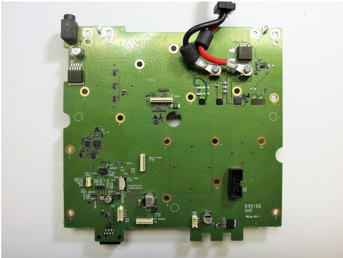
UR-FR6300 MAIN BOARD SIDE-A
