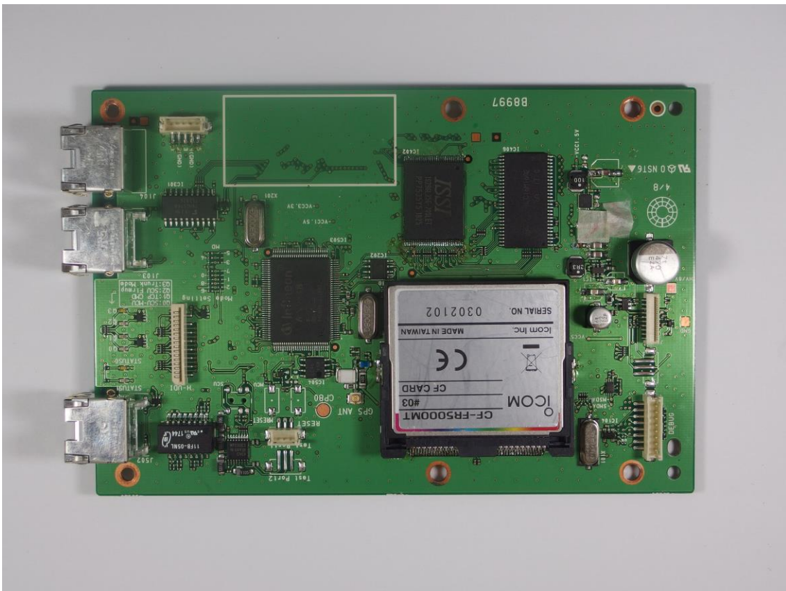
UC-FR6300 MAIN BOARD SIDE-A
