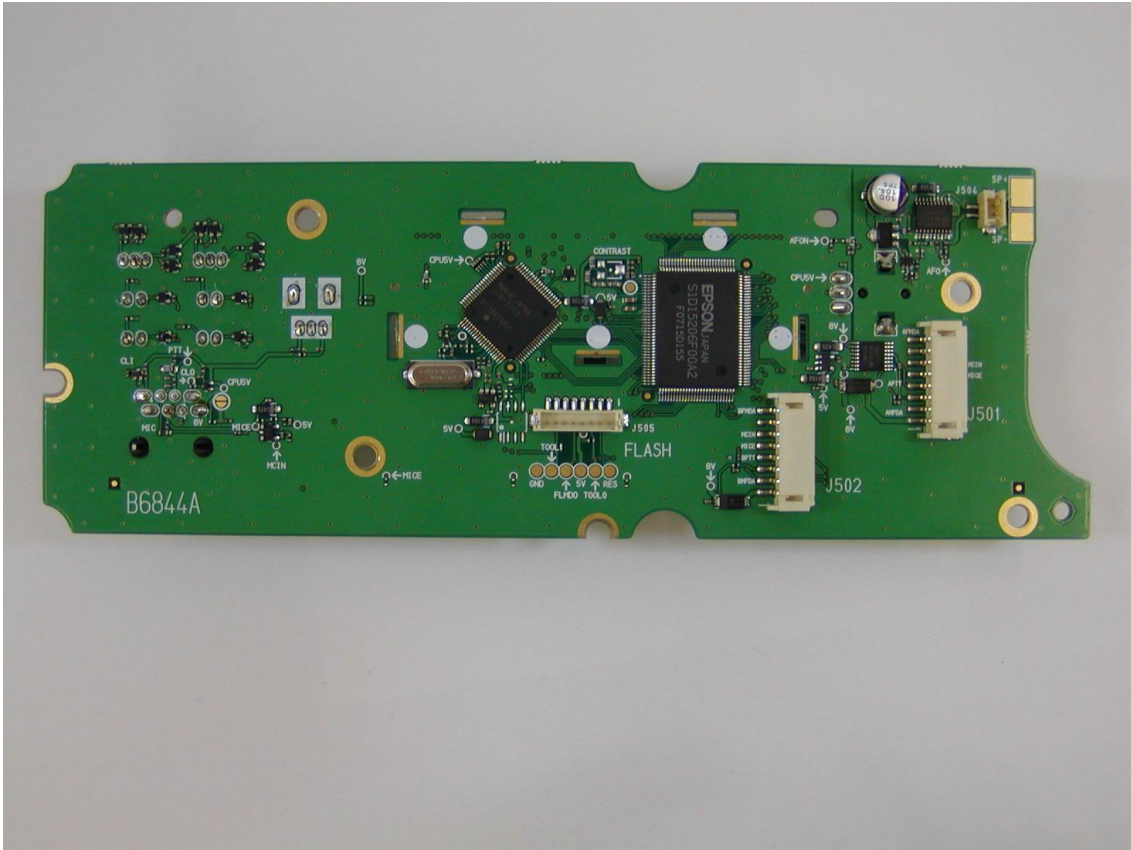
IC-FR6300 FRONT BOARD SIDE-B
