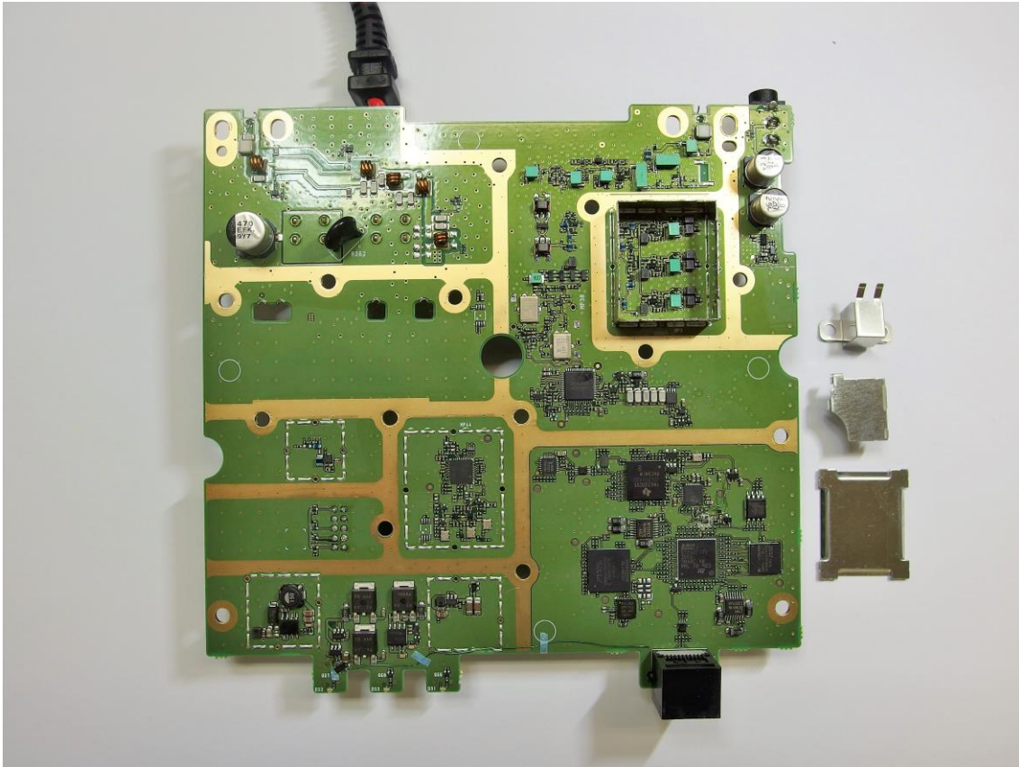
UR-FR6300 MAIN BOARD SIDE-B
