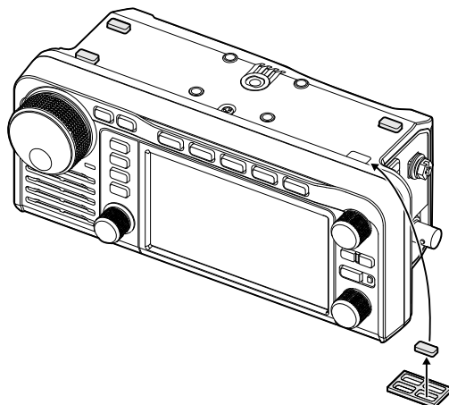
Cushion Sheet (Supplied with the transceiver)
