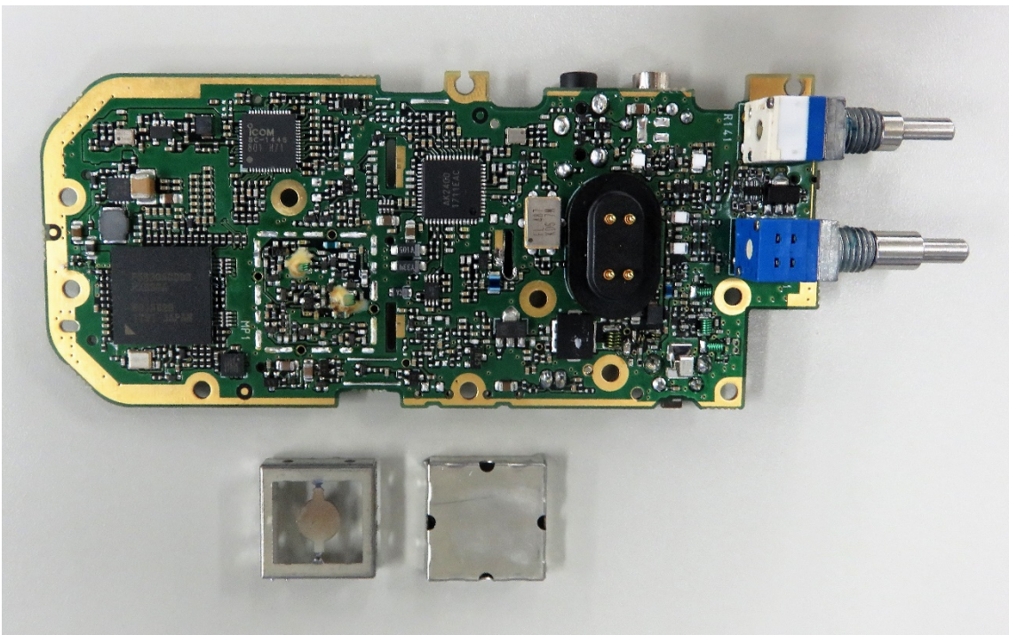
MAIN Board side-B view(IC-F2100D)
