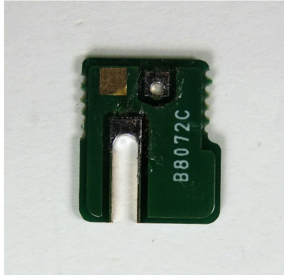
ANT Board side-A view(IC-F2100D/DS/DT)
