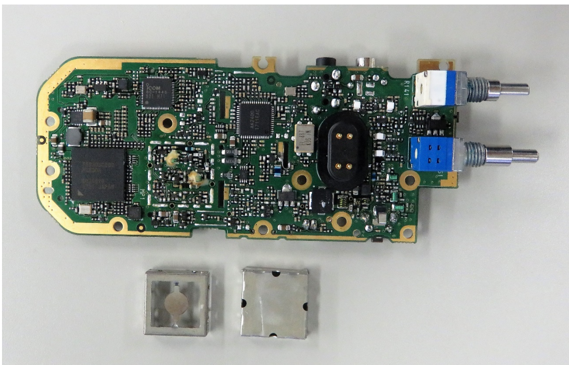
MAIN Board side-B view(IC-F2100DS)
