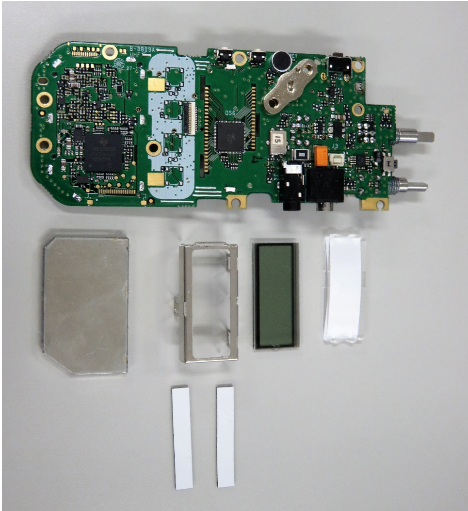
MAIN Board side-B view(IC-F2100DT)
