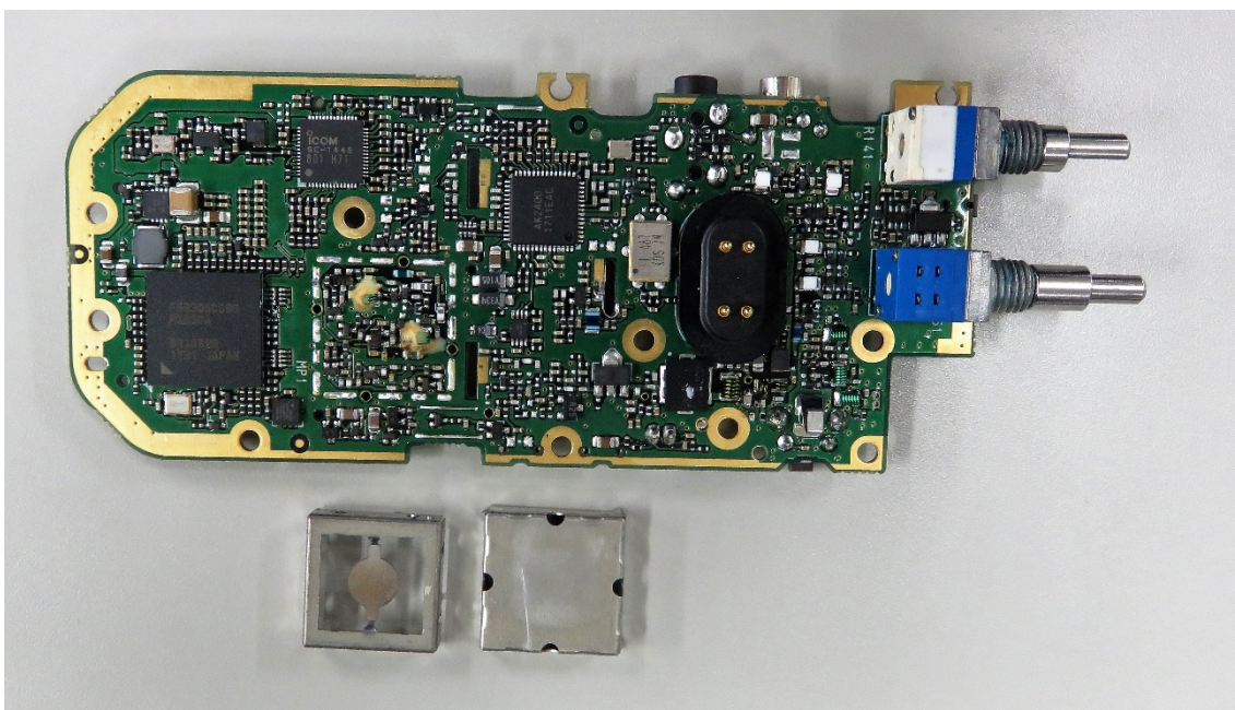
MAIN Board side-B view(IC-F2100DT)
