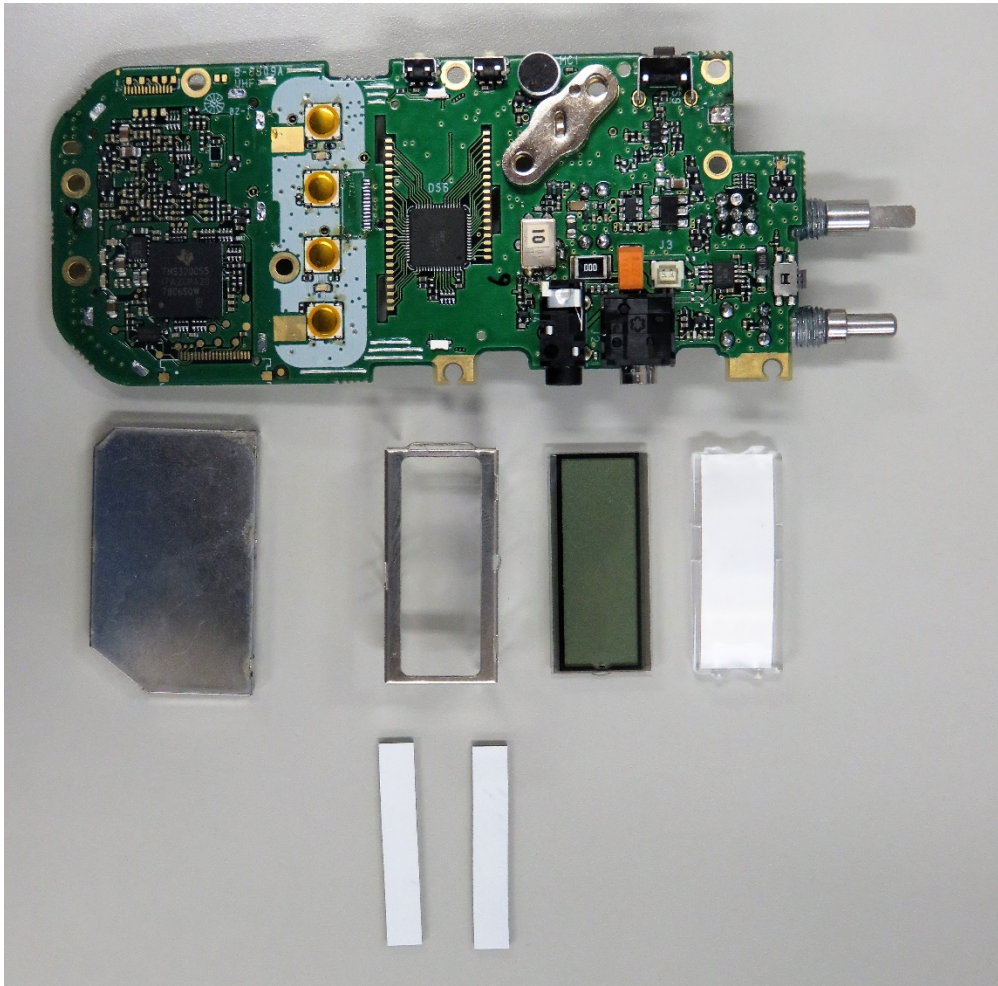
MAIN Board side-B view(IC-F2100DS)
