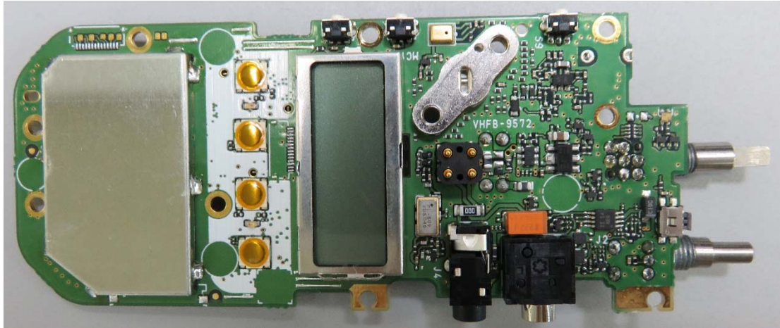
MAIN Board side-A view(IC-F1100DS)
