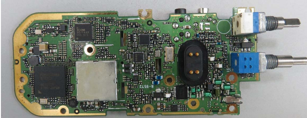
MAIN Board side-B view(IC-F1100D)
