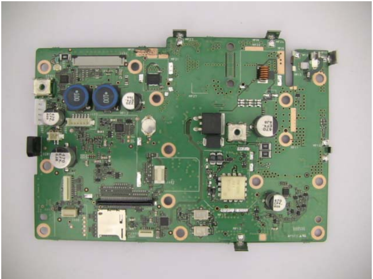
IC-F7540 MAIN UNIT A SIDE
