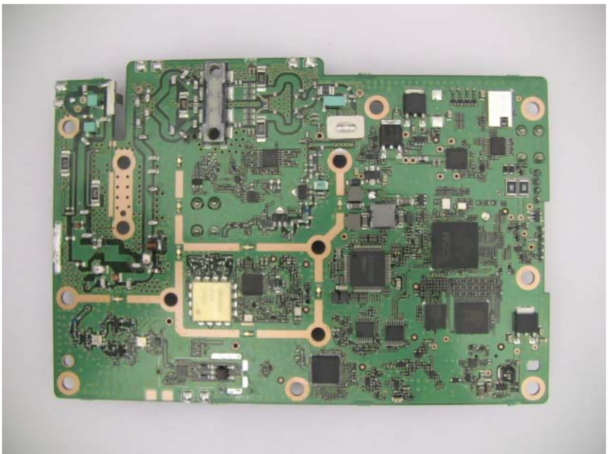
IC-F7540 MAIN UNIT B SIDE
