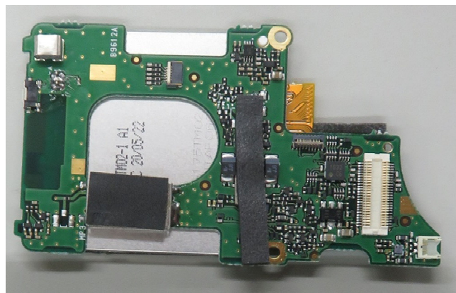
IC-F7040S/T FRONT SIDE B with LCD
