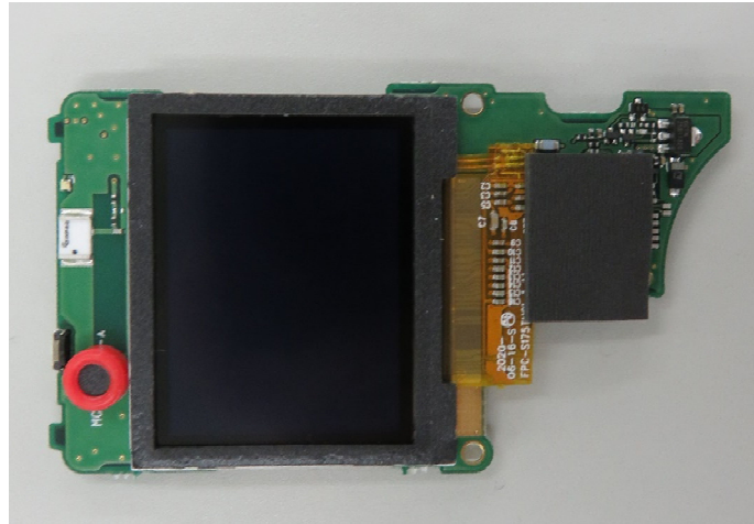
IC-F7040S/T FRONT SIDE A with LCD
