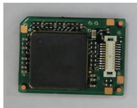
AES/DES UNIT (UT-125 FIPS) SIDE B
