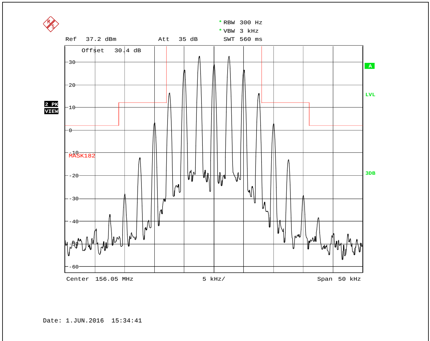
Plot 5.4.4.2.2. Emission Limitation for 156.050 MHz, 25 kHz Channel Spacing, High Power (5 W), G3E, 50 kHz Span
