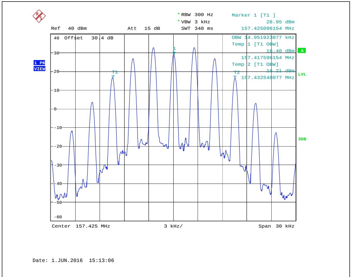
Plot 5.4.4.1.2. Occupied Bandwidth for 157.425 MHz, 25 kHz Channel Spacing, High Power (5 W), G3E
