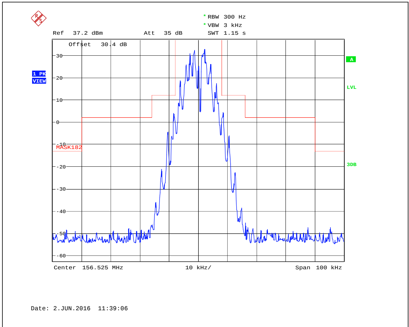
Plot 5.4.4.2.9. Emission Limitation for 156.525 MHz, 25 kHz Ch Spacing, High Power (5 W), G2B (DSC), 100 kHz Span
