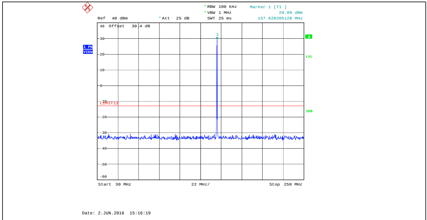
Plot 5.5.4.10. Spurious Emissions at Antenna Terminals, 157.425 MHz, 25 kHz Channel Spacing, 1 W, 30 MHz - 250 MHz
