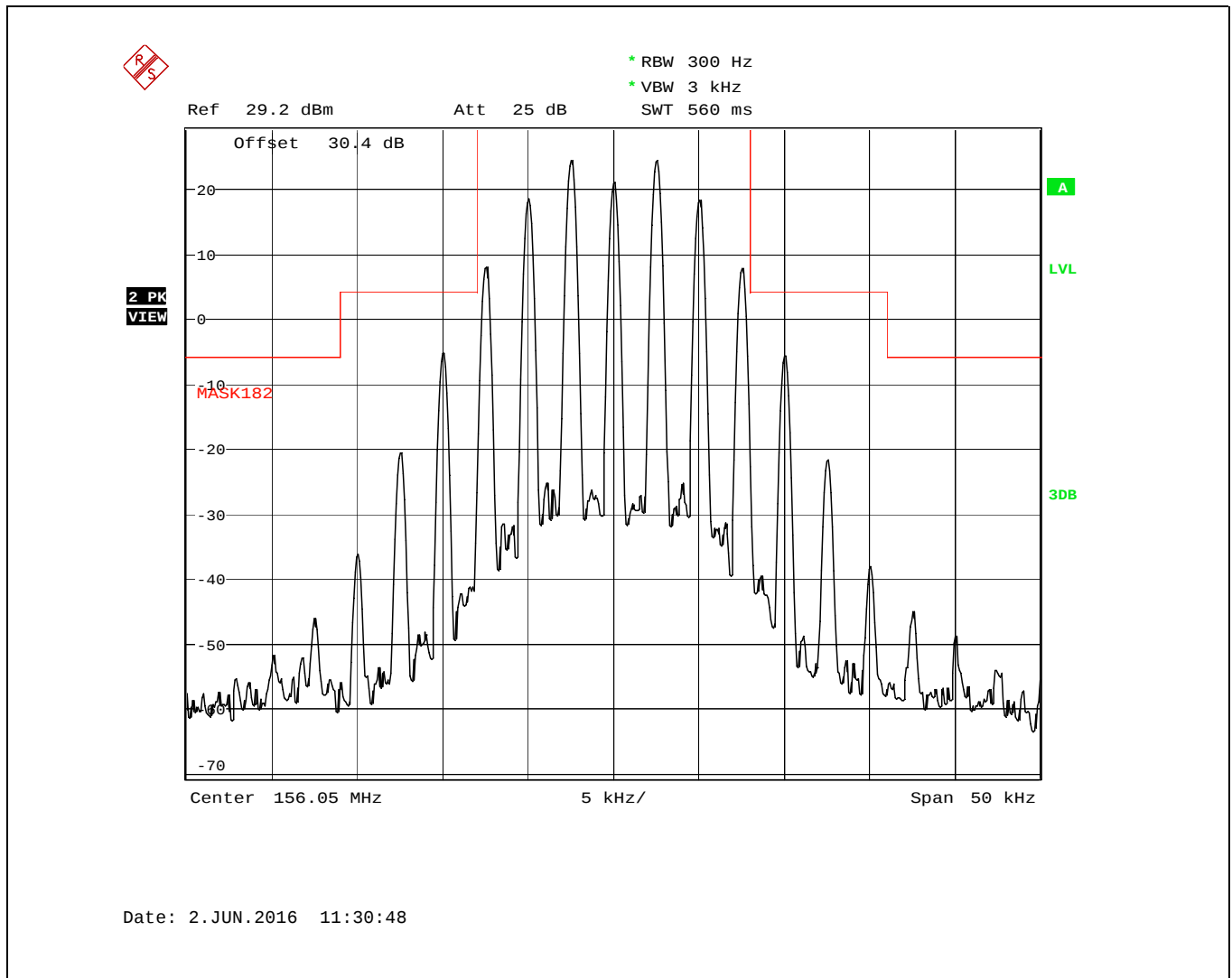
Plot 5.4.4.2.4. Emission Limitation for 156.050 MHz, 25 kHz Channel Spacing, Low Power (1 W), G3E, 50 kHz Span
