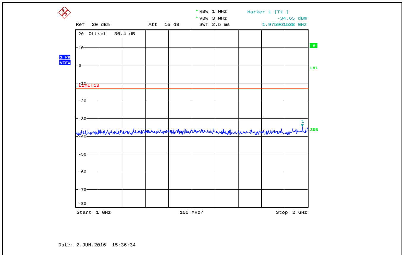
Plot 5.5.4.12. Spurious Emissions at Antenna Terminals, 157.425 MHz, 25 kHz Channel Spacing, 1 W, 1 GHz - 2 GHz
