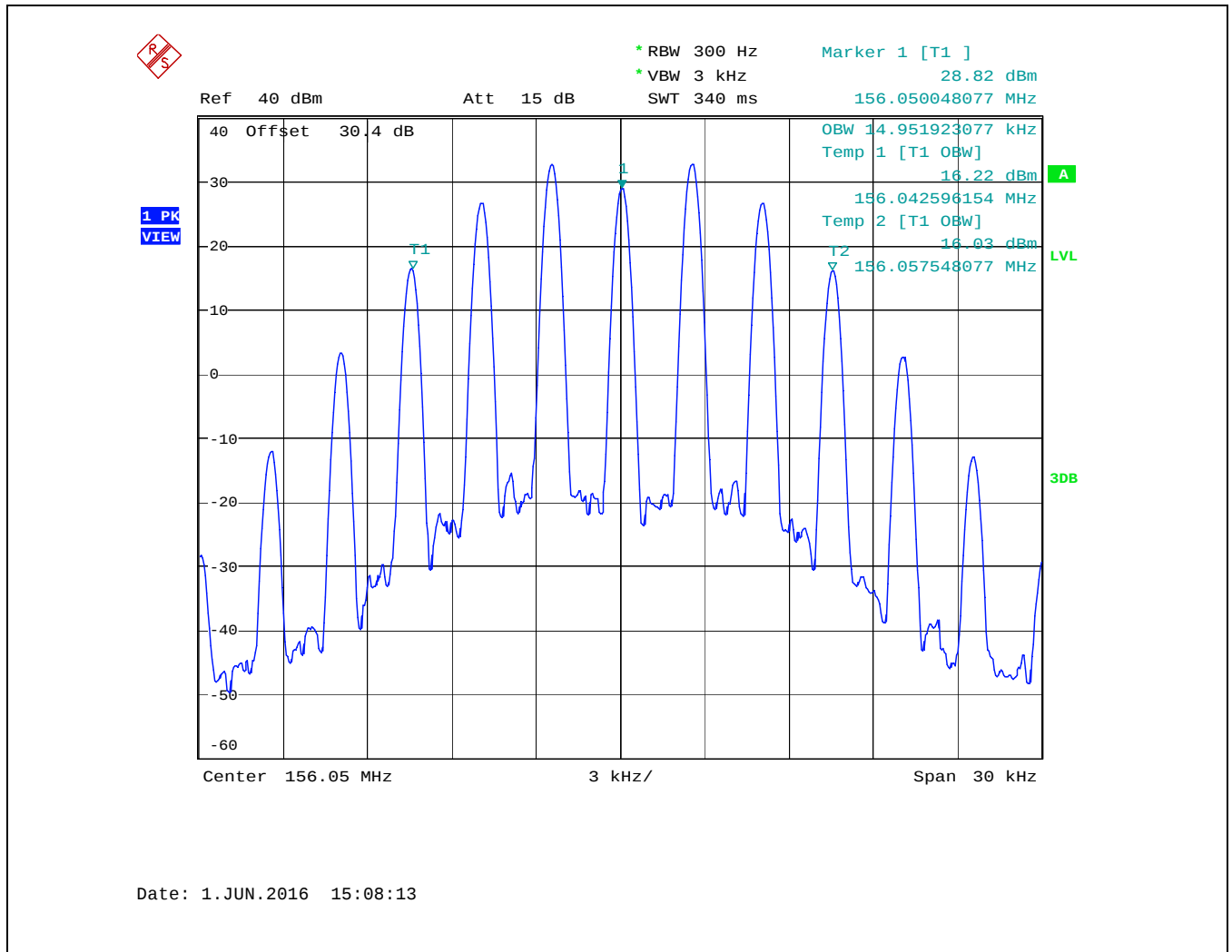
Plot 5.4.4.1.1. Occupied Bandwidth for 156.050 MHz, 25 kHz Channel Spacing, High Power (5 W), G3E
