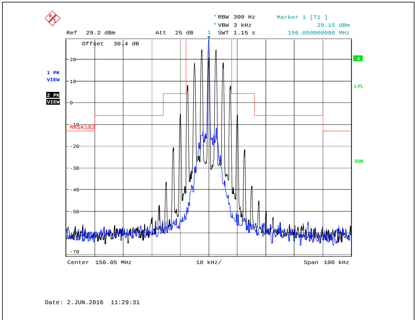
Plot 5.4.4.2.3. Emission Limitation for 156.050 MHz, 25 kHz Channel Spacing, Low Power (1 W), G3E, 100 kHz Span
