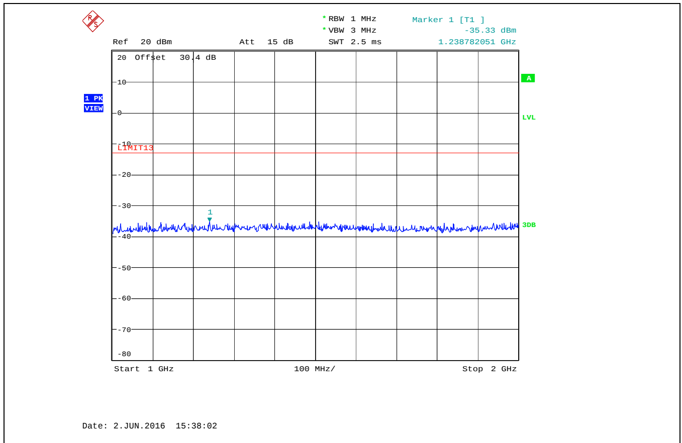
Plot 5.5.4.9. Spurious Emissions at Antenna Terminals, 157.425 MHz, 25 kHz Channel Spacing, 5 W, 1 GHz - 2 GHz
