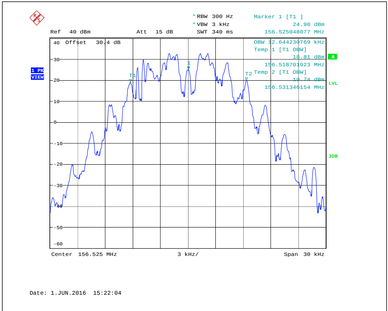
Plot 5.4.4.1.3. Occupied Bandwidth for 156.525 MHz, 25 kHz Channel Spacing, High Power (5 W), G2B-DSC
