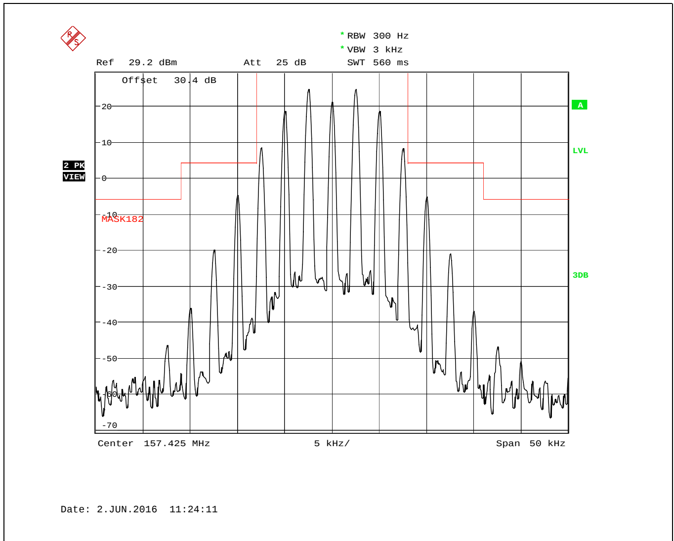
Plot 5.4.4.2.8. Emission Limitation for 157.425 MHz, 25 kHz Channel Spacing, Low Power (1 W), G3E, 50 kHz Span
