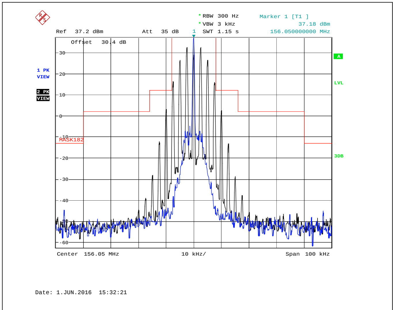
Plot 5.4.4.2.1. Emission Limitation for 156.050 MHz, 25 kHz Channel Spacing, High Power (5 W), G3E, 100 kHz Span
