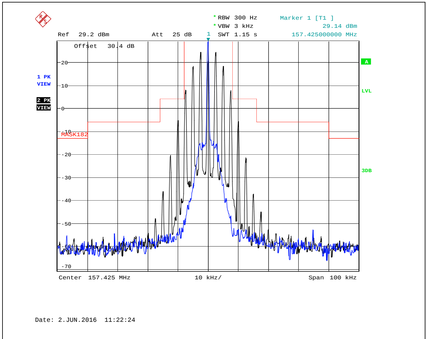
Plot 5.4.4.2.7. Emission Limitation for 157.425 MHz, 25 kHz Channel Spacing, Low Power (1 W), G3E, 100 kHz Span
