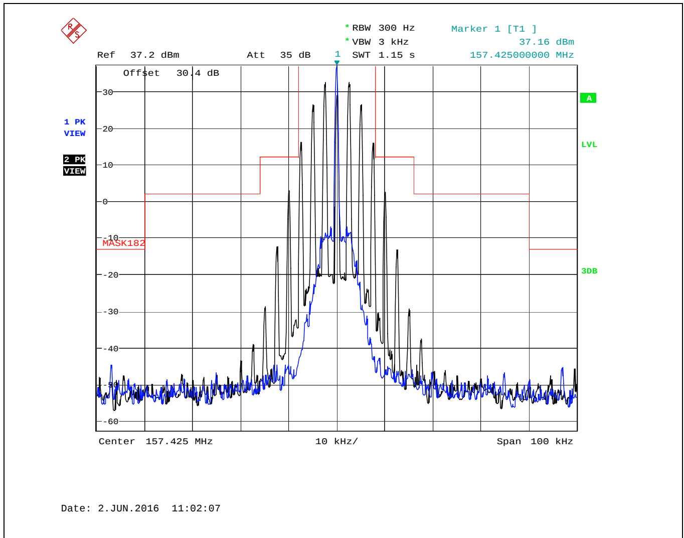
Plot 5.4.4.2.5. Emission Limitation for 157.425 MHz, 25 kHz Channel Spacing, High Power (5 W), G3E, 100 kHz Span
