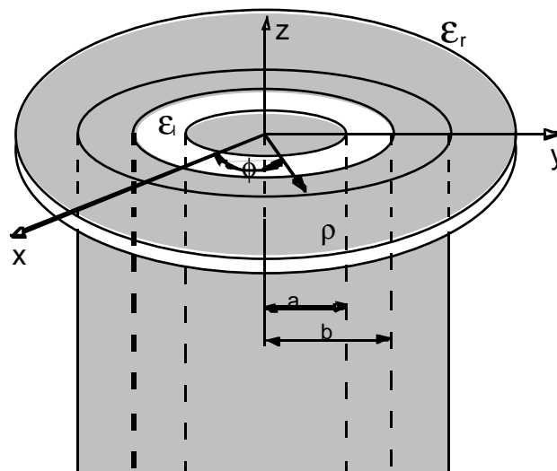
Figure Error! Reference source not found.. An open-ended coaxial probe with inner and outer radii a and b , respectively
